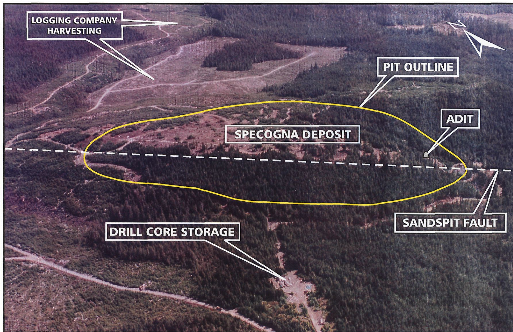
MISTY MOUNTAIN GOLD LIMITED HARMONY GOLD PROJECT SPECOGNA DEPOSIT
