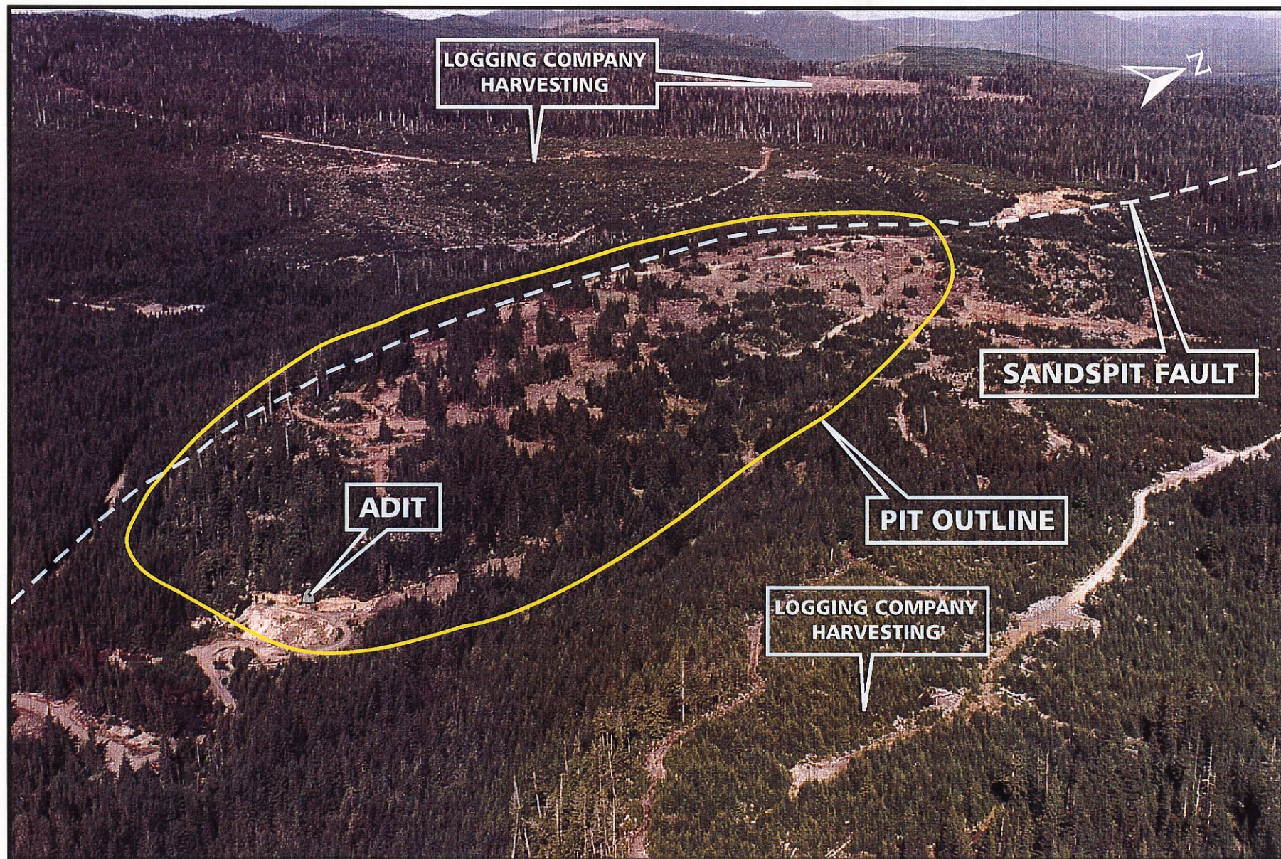
MISTY MOUNTAIN GOLD LIMITED HARMONY GOLD PROJECT SPECOGNA DEPOSIT
