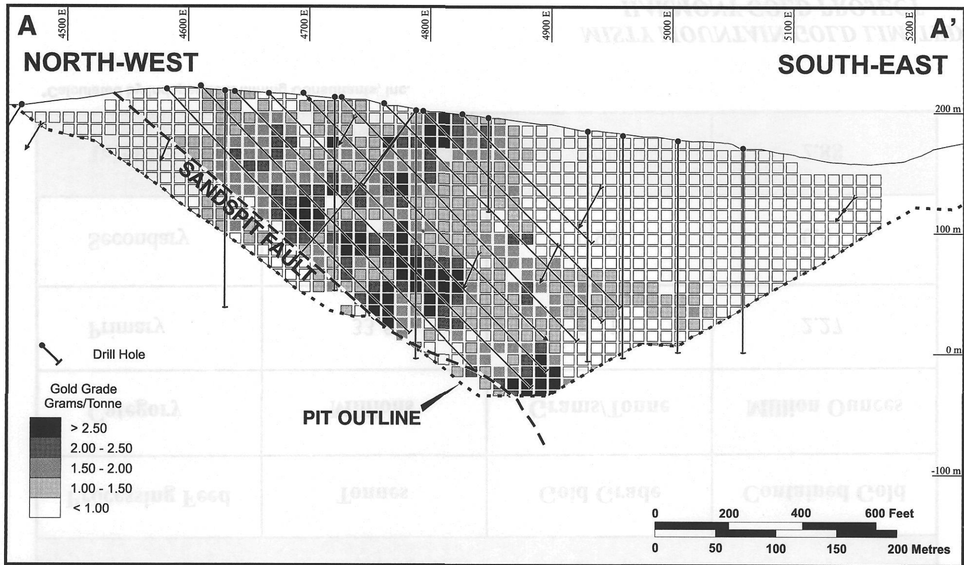
MISTY MOUNTAIN GOLD LIMITED HARMONY GOLD PROJECT SECTION A - A' GRADE MODEL
