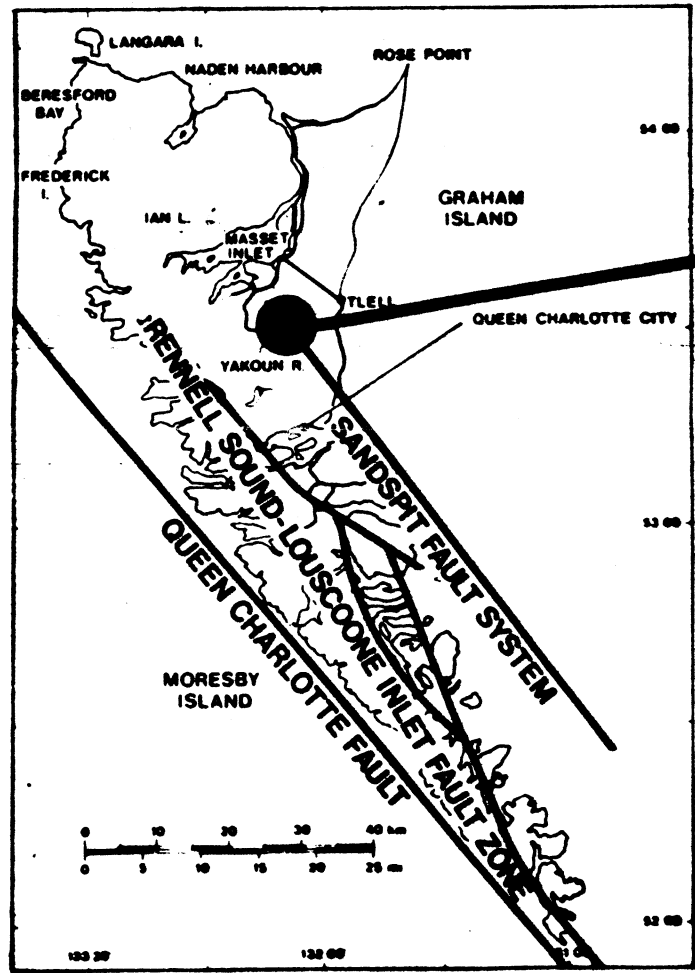
Structural setting of the Queen Charlotte Islands (modified after Yorath and Hyndman, 1983)
