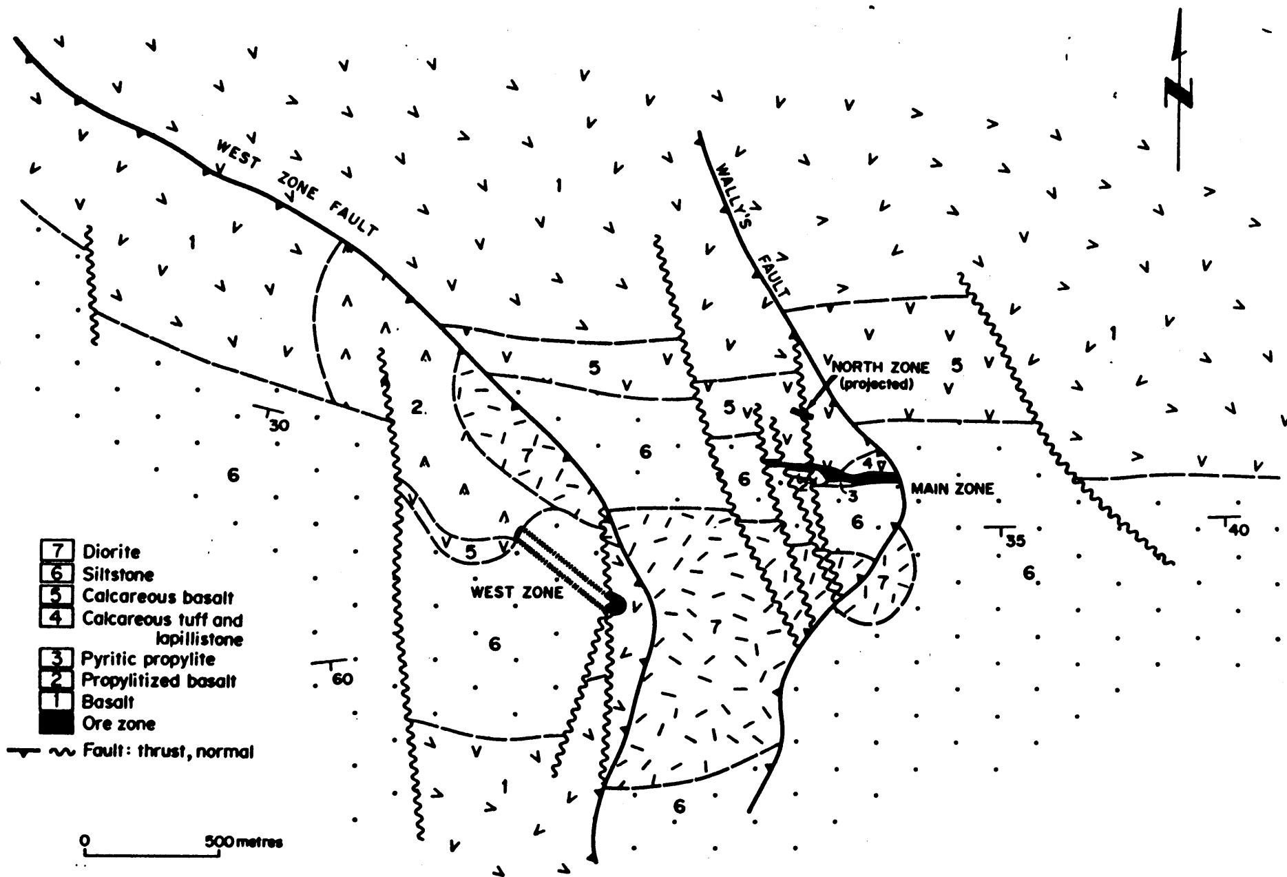
QUESNEL RIVER PROPERTY - GEOLOGY
