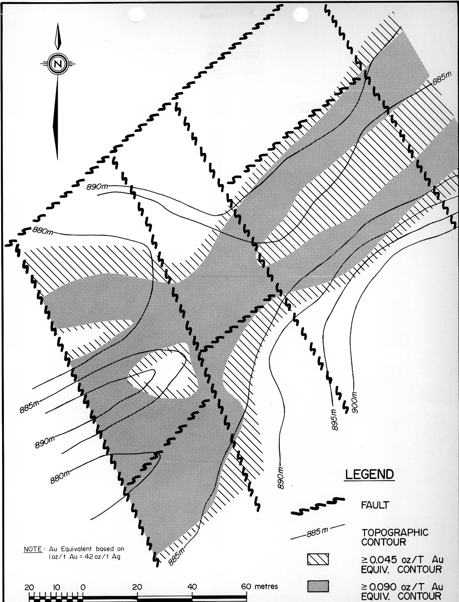
PRE-DEFORMATION GRADE and TOPOGRAPHIC CONTOUR MAP for BASE of D-ZONE, DAGO ZONE
