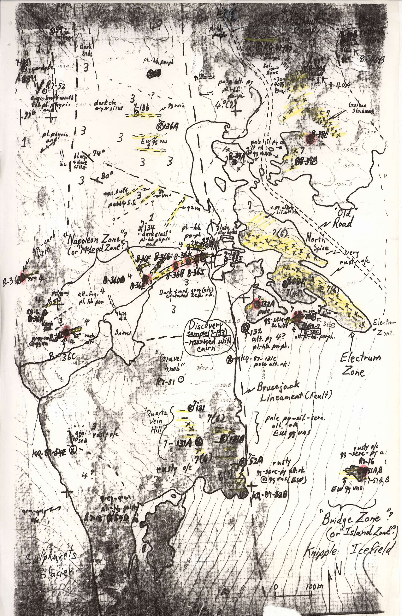
Sketch Map Showing Rvt Sample Locations in Vicinity of Nappe R.V. Kir
