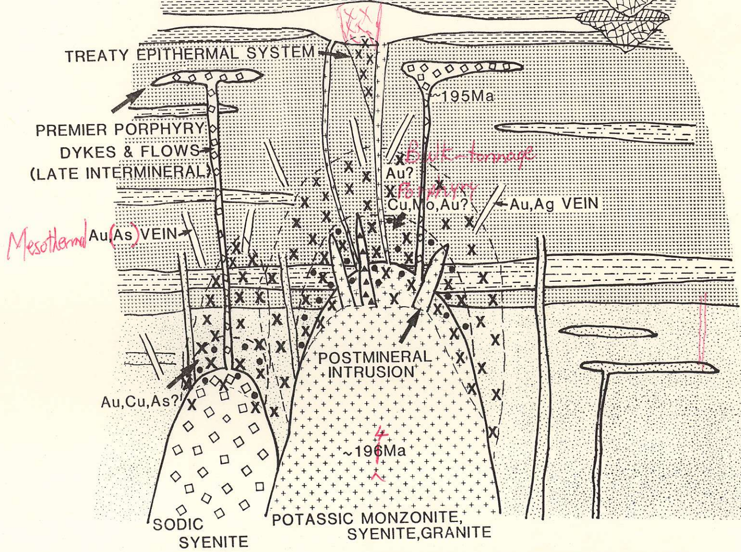
SULPHURETS SCHEMATIC STRATIGRAPHY AND SYNINTRUSIVE, SYNVOLCANIC MINERAL DEPOSITS
