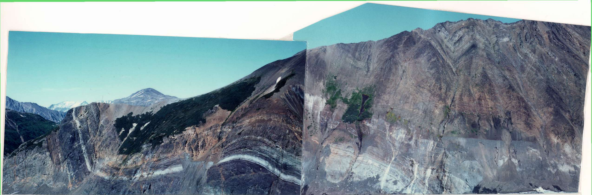
Unuk River?, Betty Creek, Mount Dilworth, Salmon River and Bowser Lake sandstone and mudstone, north side of South Treaty Glacier
