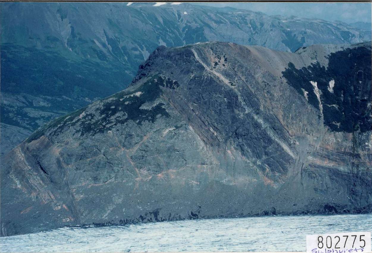
Treaty Glacier: Betty Creek, Mount Dilworth and Salmon River Formations
