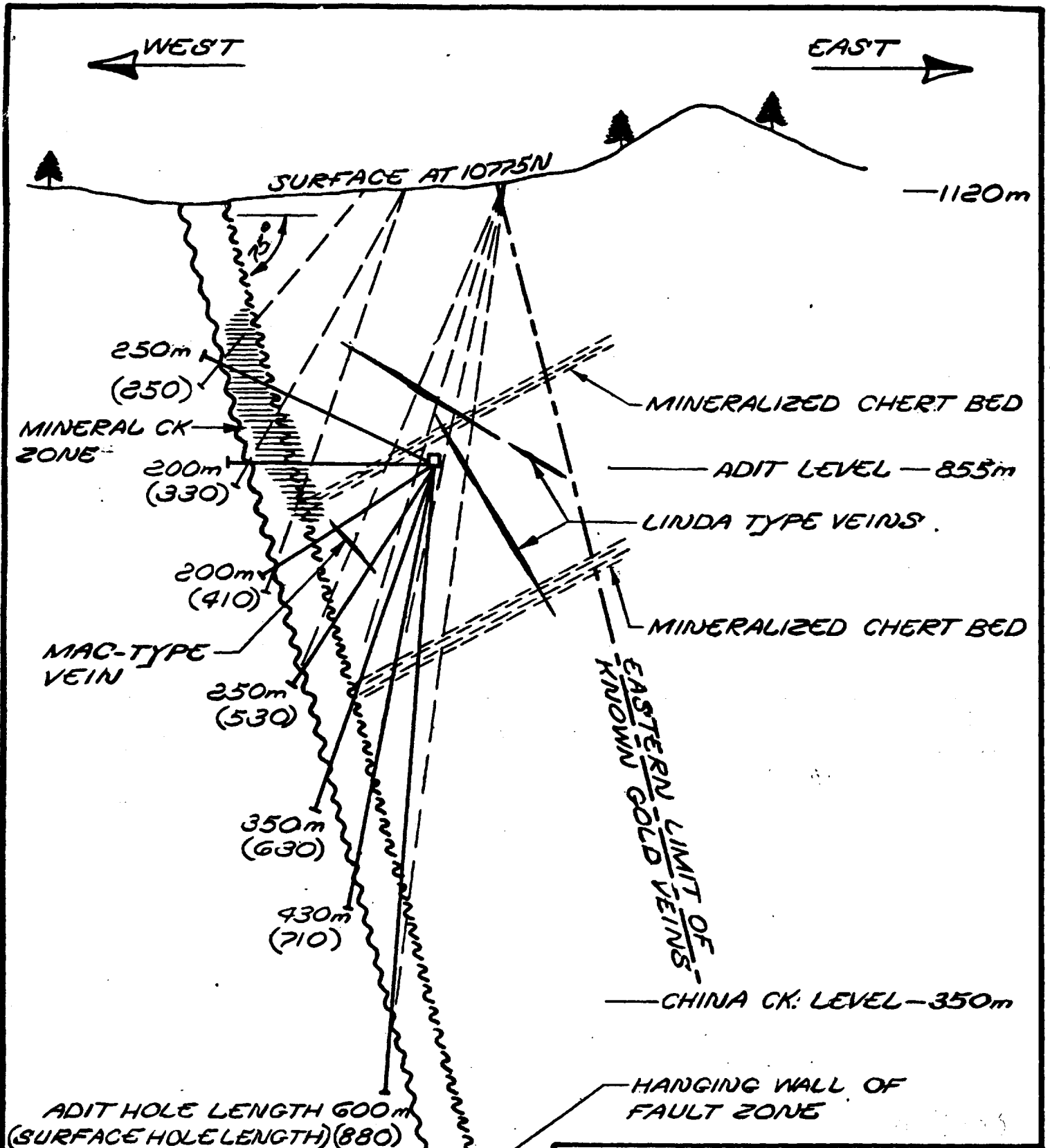
FIG. 2 DEBBIE/YELLOW PROJECTS COMPOSITE CROSS SECTION EXPLOATION TUNNEL 0 100 200 300 METERS R.R.W. FEB 88
