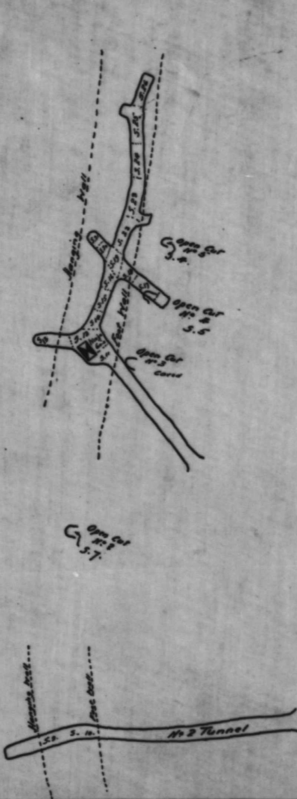
Plan of Workings Wisconsin & Lucky Strike Claims. Situated near Middle Creek, B.C. Scale = 30 feet to 1 inch. S = Sample.
