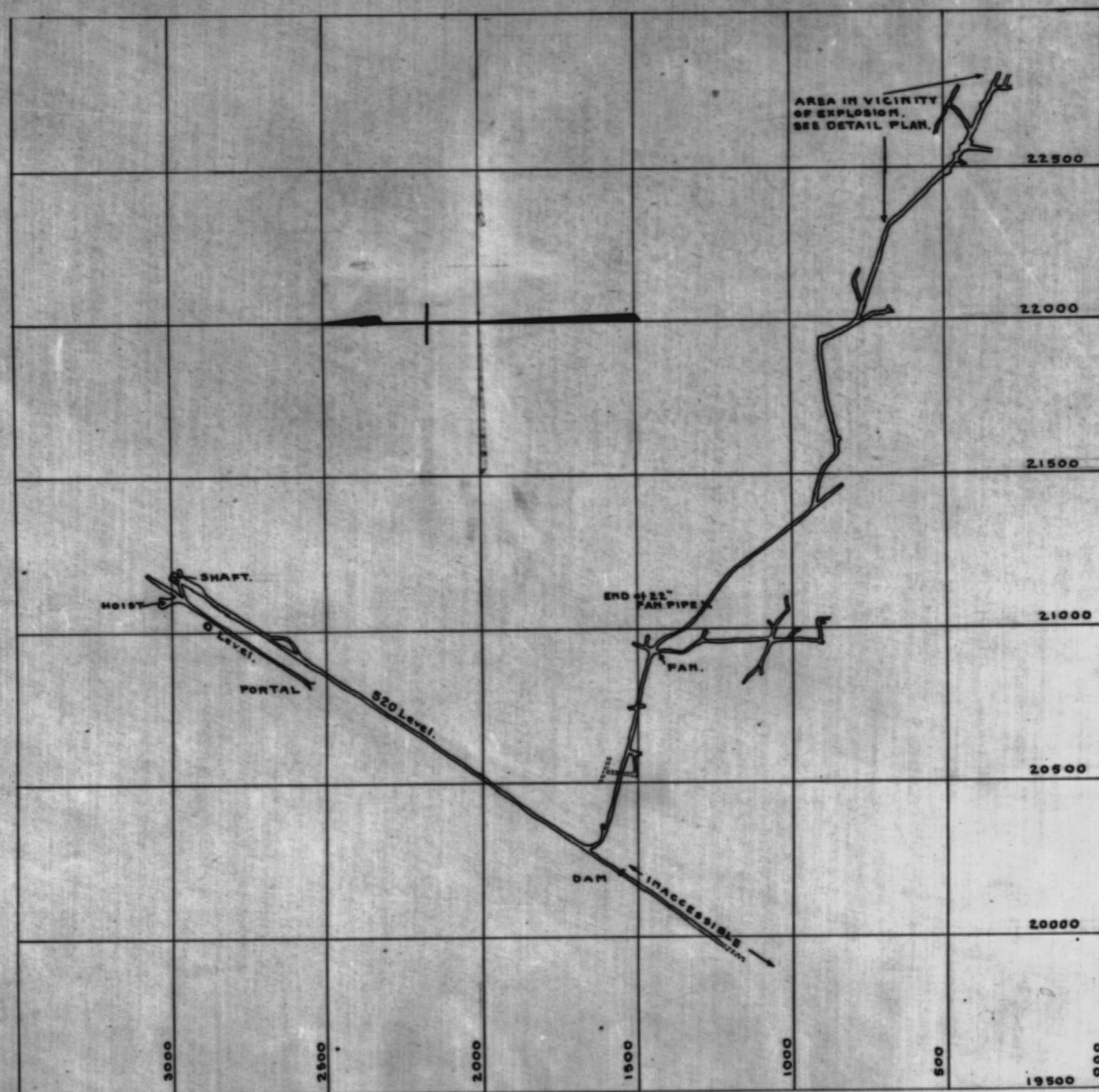
PLAN of PACIFIC EASTERN GOLD MINES. LILLOOET M.D. SCALE 1"=300' To accompany Report of Investigation into Explosion on Aug. 18, 1947. H.C.H.
