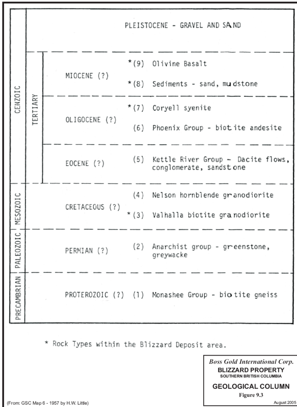
Figure 9.3. Geologic Column for Blizzard Property Area.
