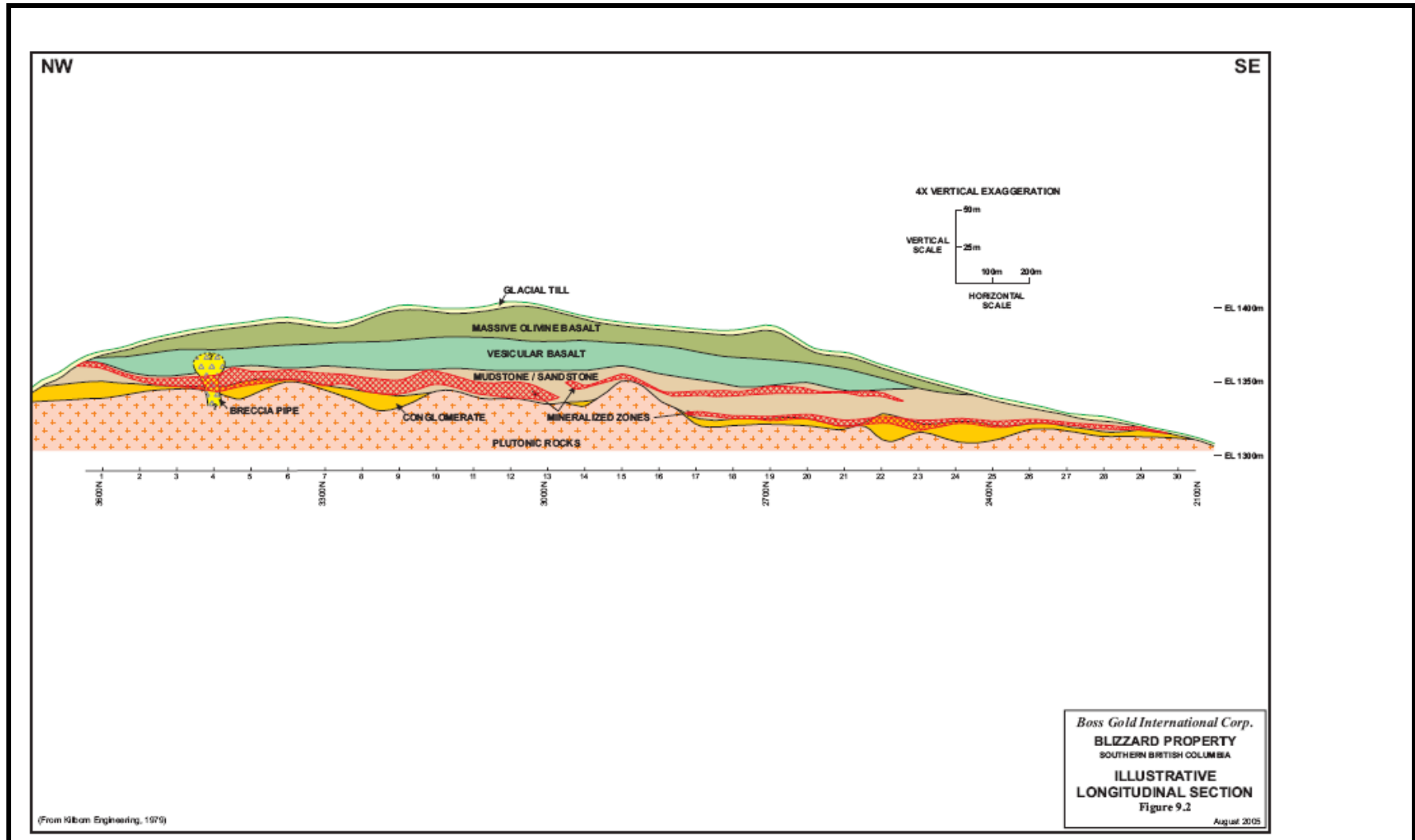
Figure 9.2 Illustrative Longitudinal Section of Blizzard Deposit.
