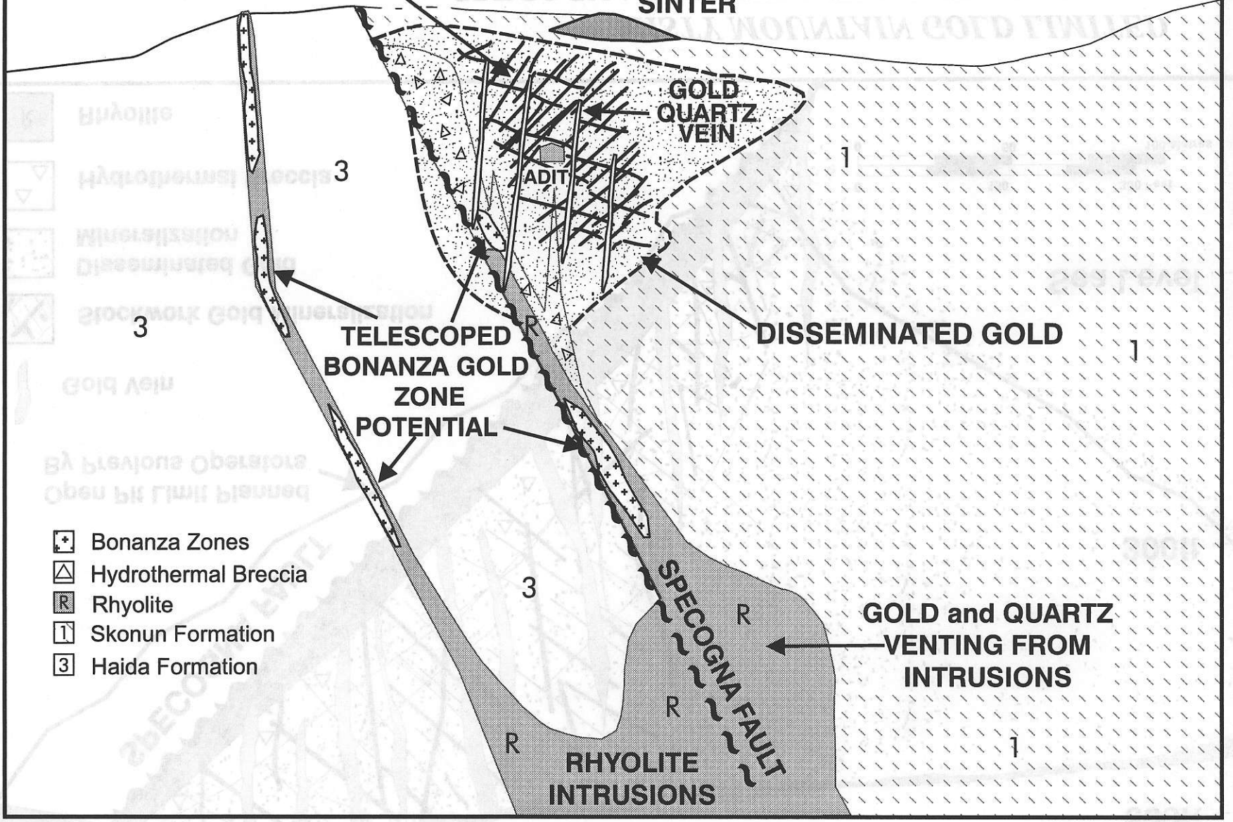
MISTY MOUNTAIN GOLD LIMITED SPECOGNA DEPOSIT MODEL
