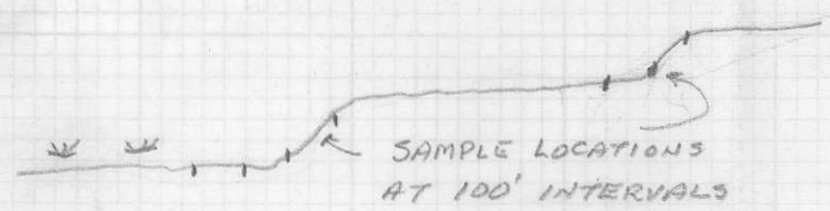
PROFILE FROM SWAMP TO PINE FLATS
