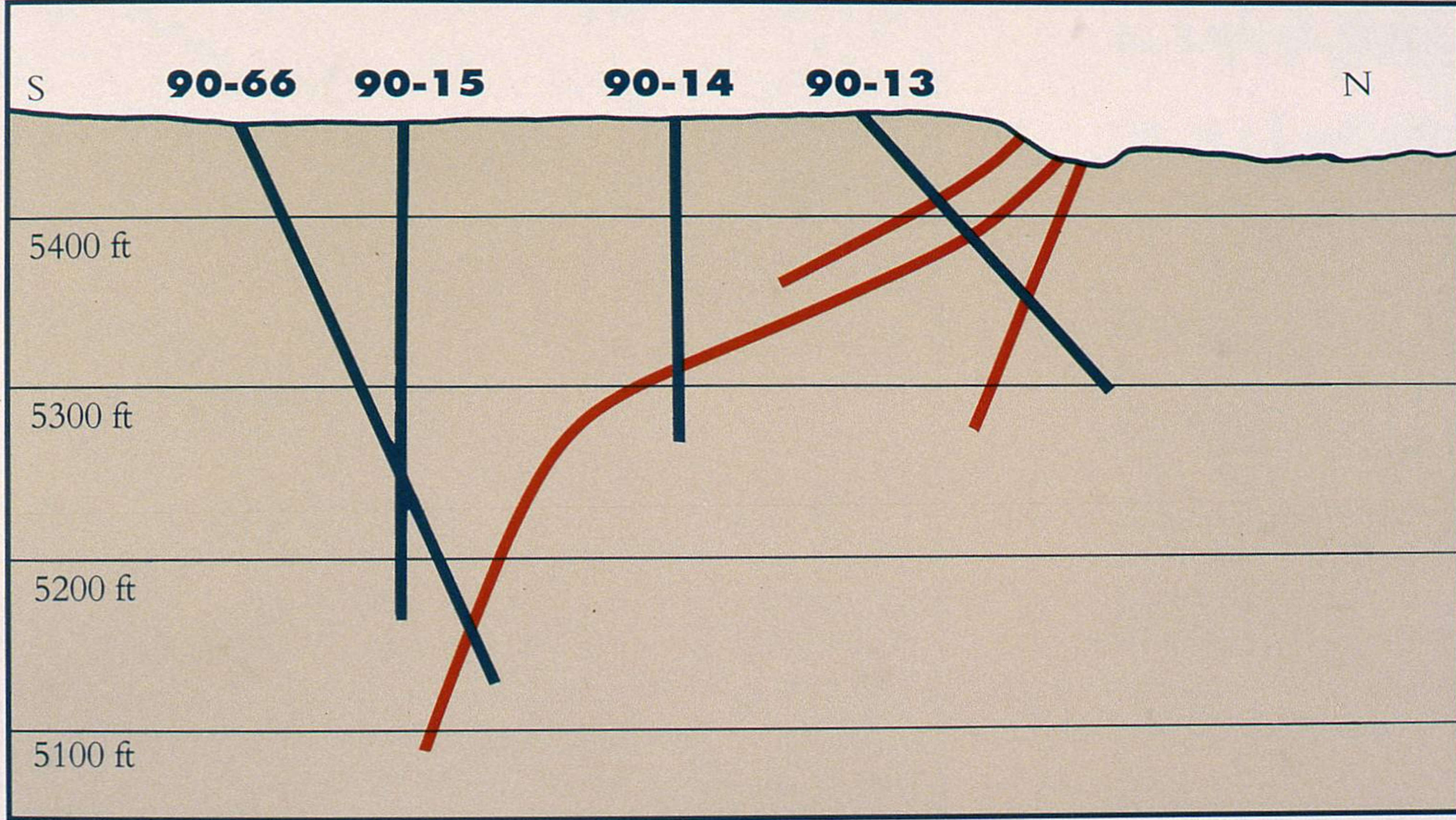
Siwash North Diamond Drill Section A
