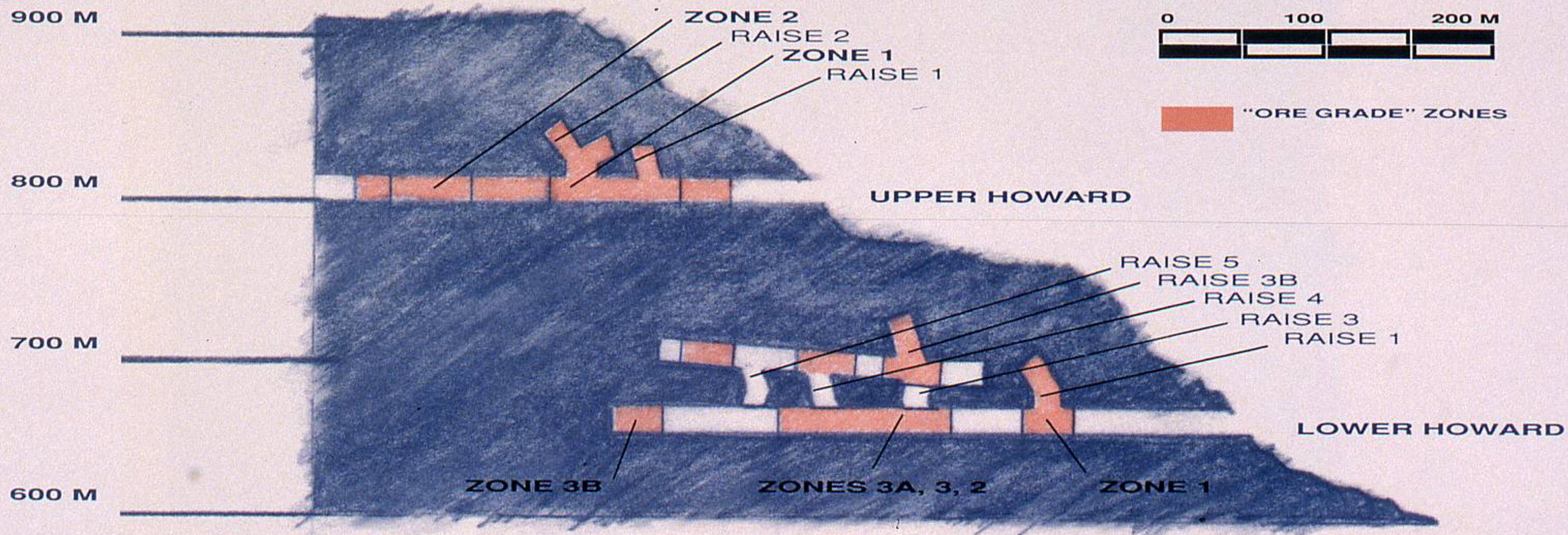
Long section view of the Howard drift showing ore intersections to date.
