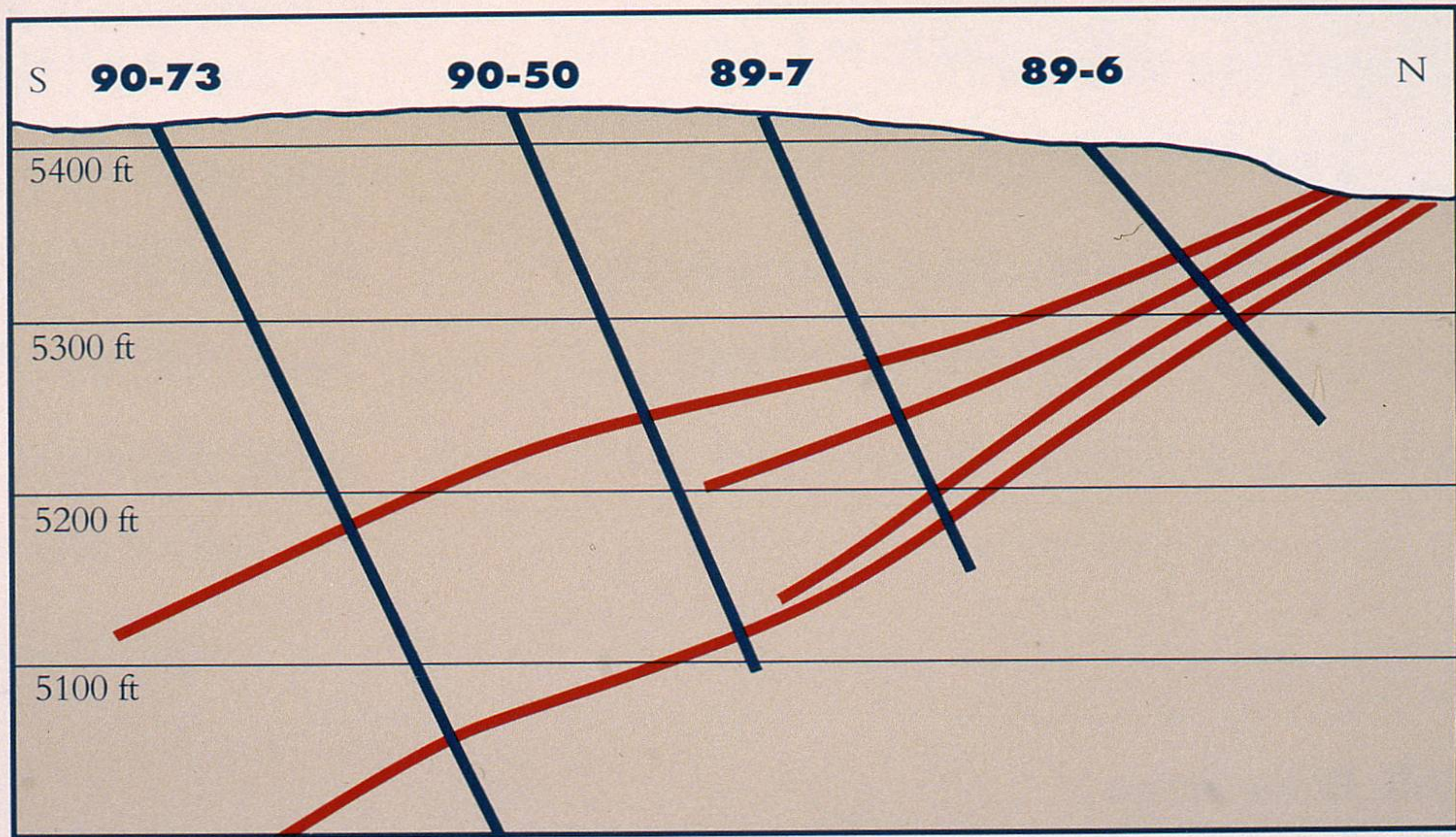
Siwash North Diamond Drill Section B
