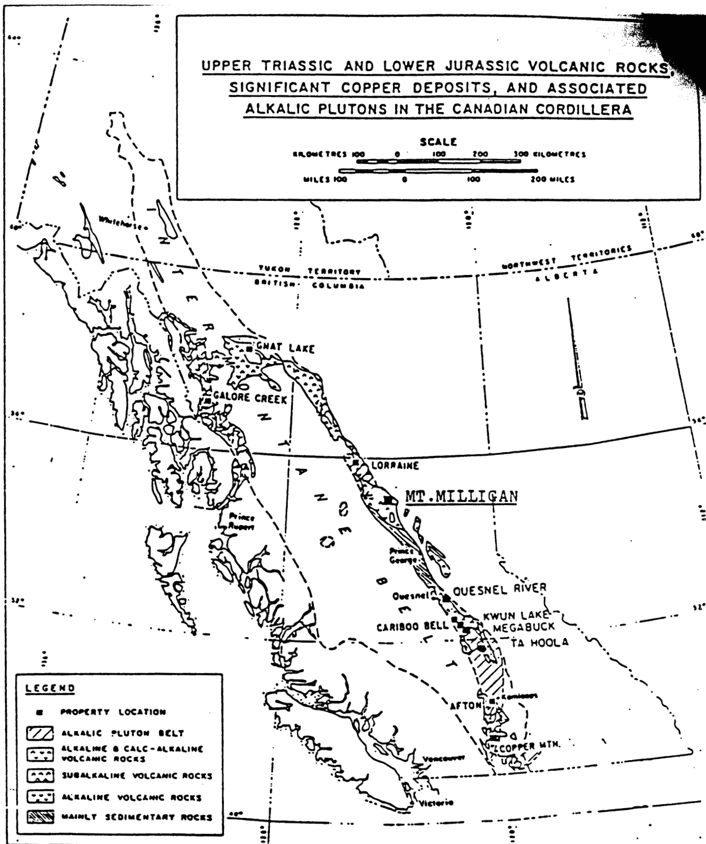
FIGURE 1 — Upper Triassic and Lower Jurassic volcanic rocks, significant copper deposits and associated alkalic plutons in the Canadian Cordillera.
