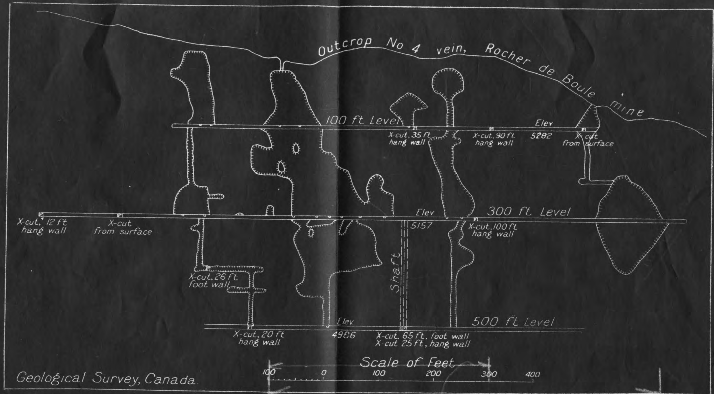
Figure 2. Stope elevations projected on plane of vein No. 4, Rocher Déboulé mine, 1917, Rocher Déboulé mountains, British Columbia. (By courtesy of management).
