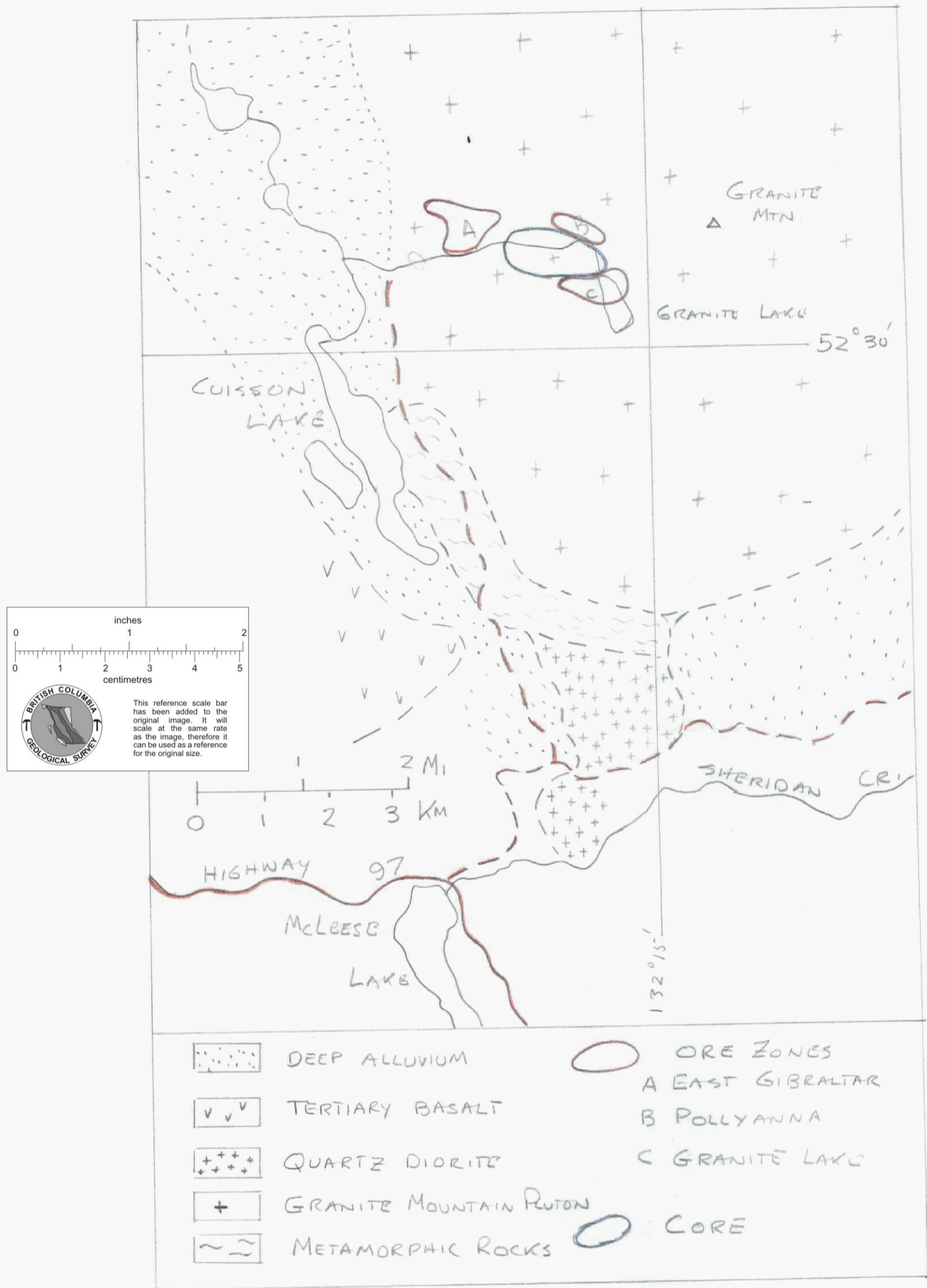
FIG 17 GEOLOGICAL SKETCH OF GIBRALTAR AREAS
