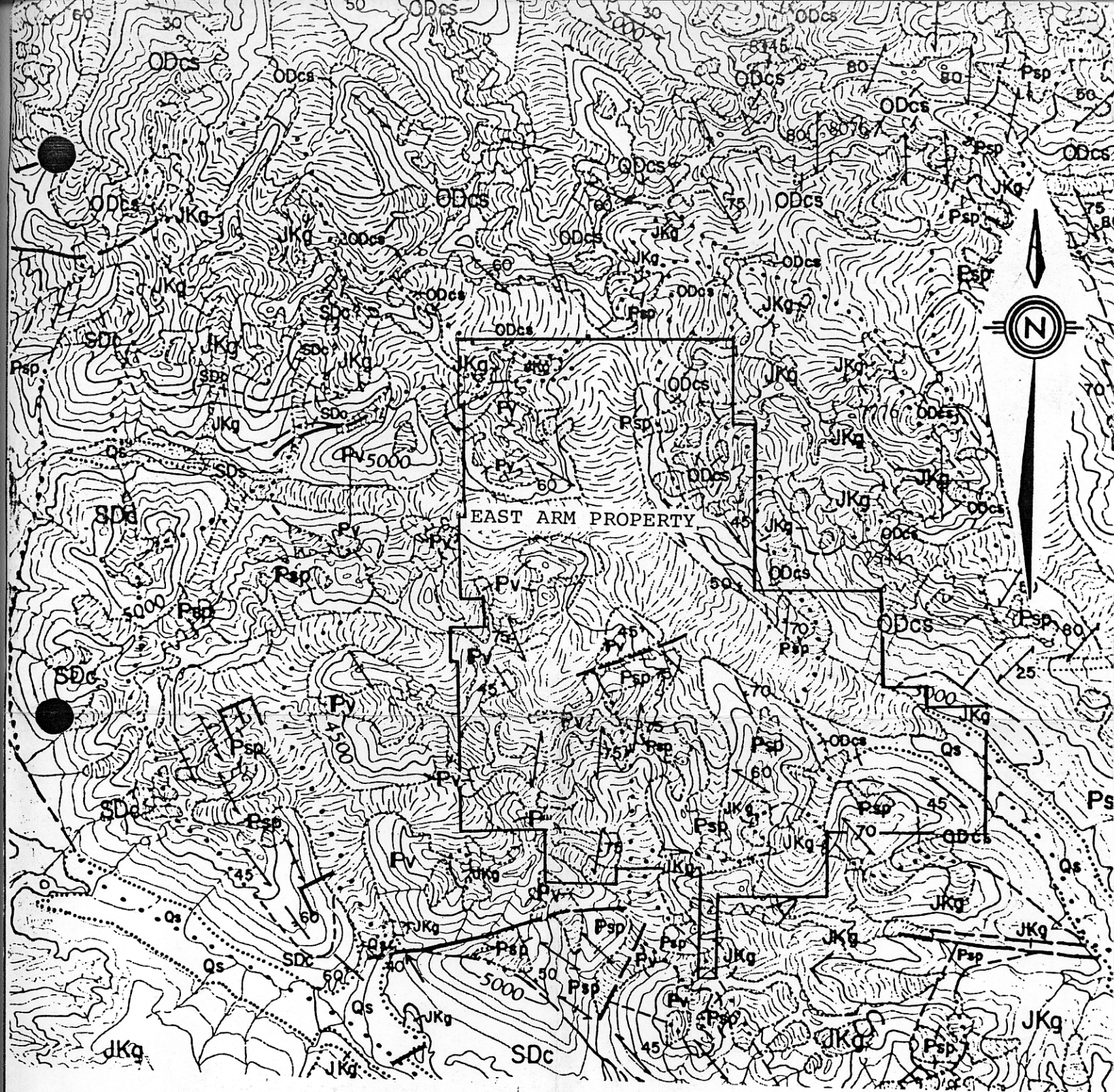
FIGURE 3 GEOLOGY OF THE TATSHENSHINI RIVER MAP AREA (114P) (from G.S.C. Open File 926)
