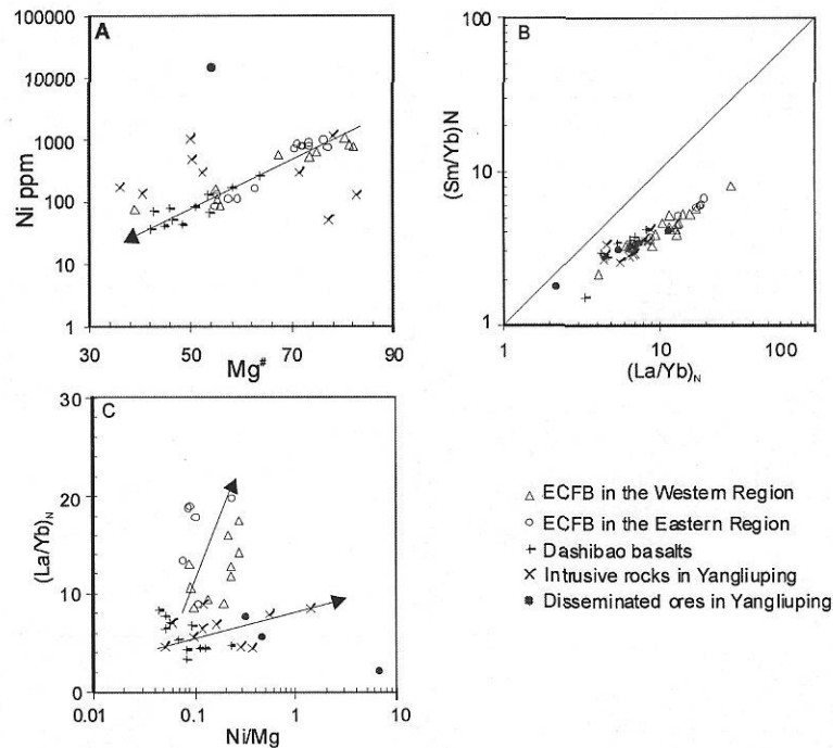
Figure 3. A) Variation diagram for Ni (ppm) against Mg^* for the ECFB and intrusive rocks (fields of high-Ti and low-Ti based on Lightfoot et al., 1993). Mg^* = Mg/(Mg + Fe_{total}) . B) Plot of (Sm/Yb)_c versus (La/Yb)_c for the ECFB, (Sm/Yb)_c and (La/Yb)_c are chondrite-normalized ratios of rare earth elements. The values of the rare earth element of the chondrite are from Tabor and McLennan (1985). C) Variation diagrams of (La/Yb)_n versus Ni/Mg for the ECFB, intrusive rocks and sulfide ores.
