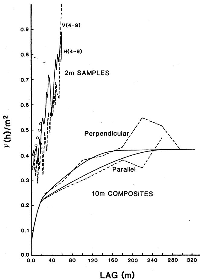
Figure 6. Horizontal semi-variograms, Cinola Gold Deposit. Two lower experimental curves, for directions parallel and perpendicular to the mean quartz vein orientation (strike 028 degrees, dip vertical) are fitted by smooth nested spherical models with a common sill and represent a model for 10m composites. The two upper jagged experimental curves are based on vertical and horizontal chip samples (over 2m) from an underground exploration adit and are fitted by a 2m model (open circles) consistent with the accompanying 10m model
