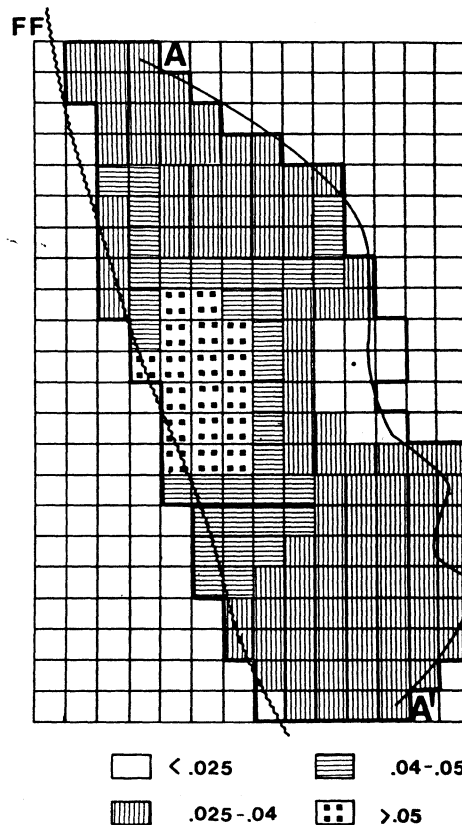
Figure 9. Example of generalized grade distribution for 30m blocks, 110m level, Cinola Gold Deposit. Results based on kriging using the isotropic two-dimensional semi-variogram model
