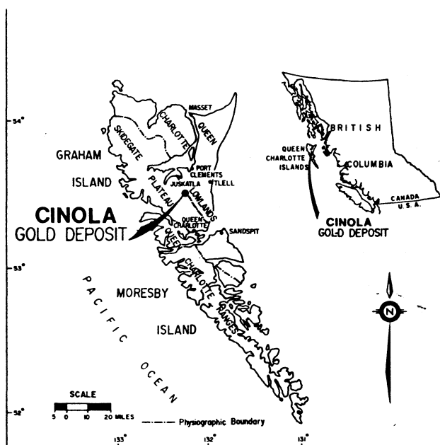
Figure 1. Location map of Cinola Gold Deposit
