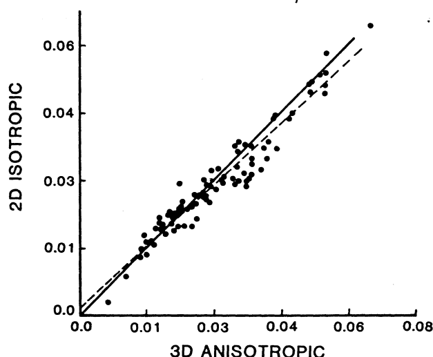
Figure 7. Comparison of block grades kriged by two different semi-variogram models for 30m blocks, 110m level, Cinola Gold Deposit. The two models are a two-dimensional isotropic model and a three-dimensional anisotropic model
