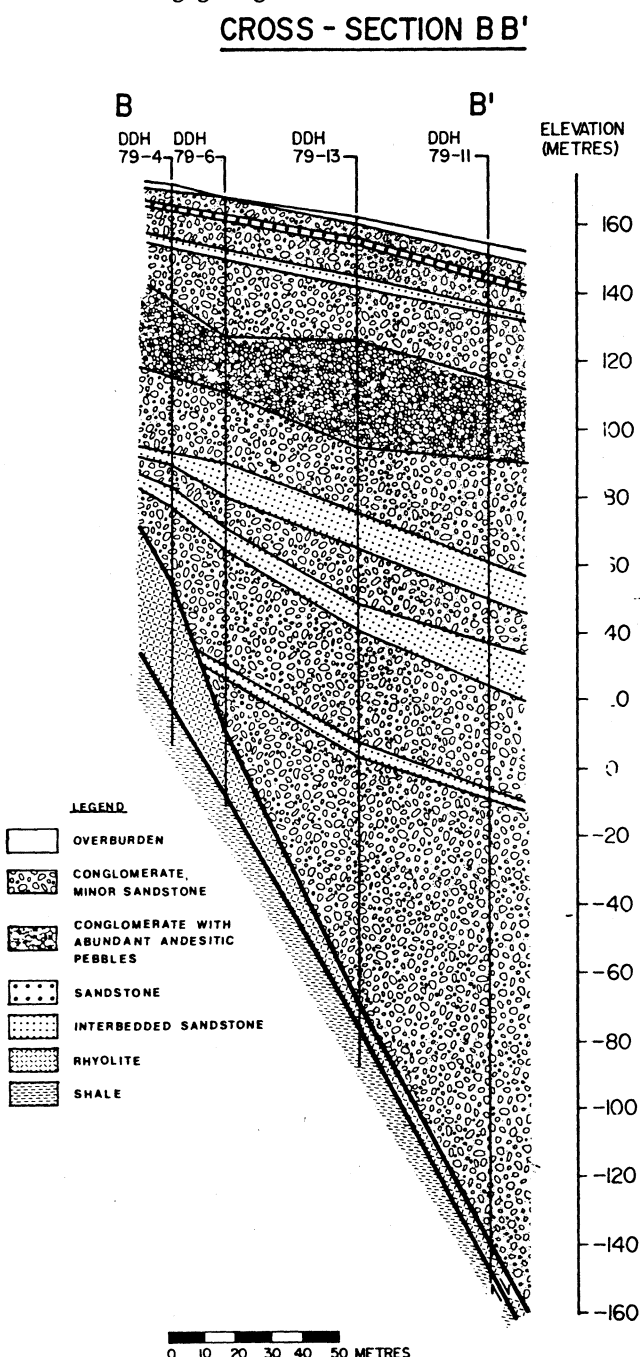
Figure 2. East-west cross-section demonstrating drill hole spacing and general geological character of the Cinola Gold Deposit. Heavy line at base of rhyolite unit is the Footwall fault below which negligible gold mineralization occurs
