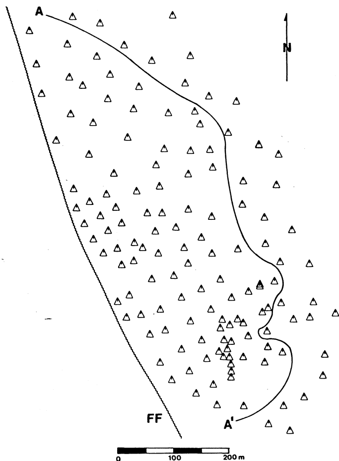
Figure 5. Collar locations of drill holes with assay data used in this study. FF is the surface trace of the Footwall fault which dips moderately to the east and forms the western and lower boundary to the main zone of gold concentration. The sinuous line, AA' separates the main zone of gold mineralization from an easterly zone of intense argillic alteration
