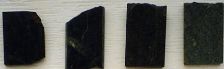
PROPYLITIC
