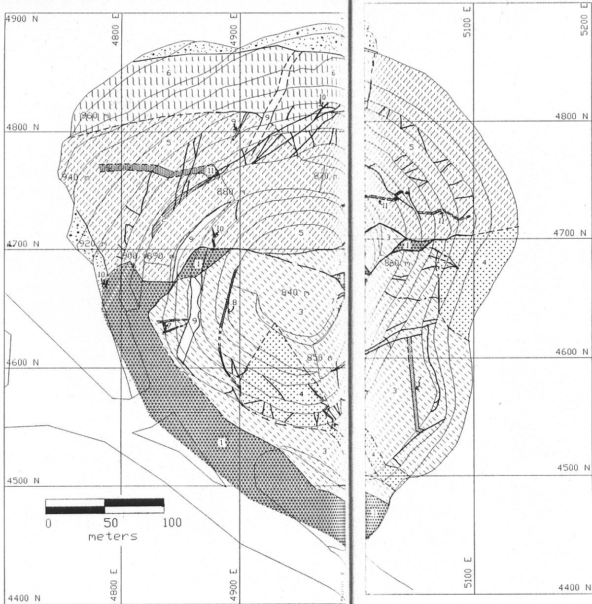
Figure 1. Geology of the Ajax West pit.
