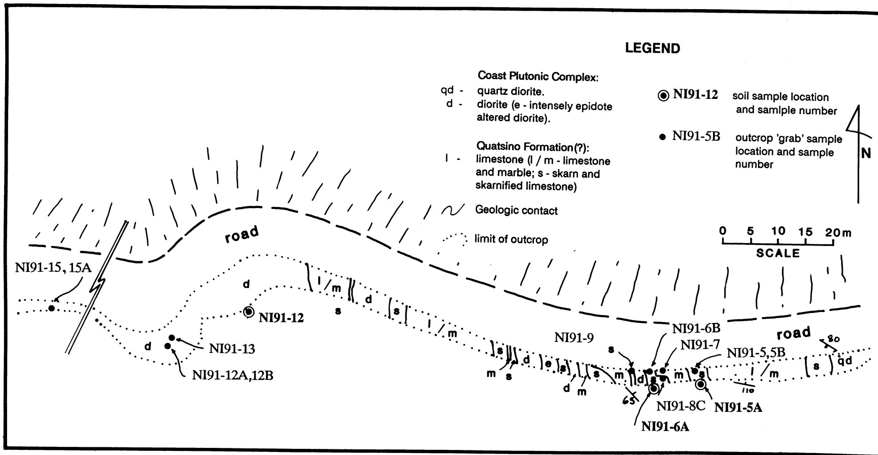
Figure B-x-x. Geological plan map of skarn occurrence, central Nelson Island. Sample locations are also shown.
