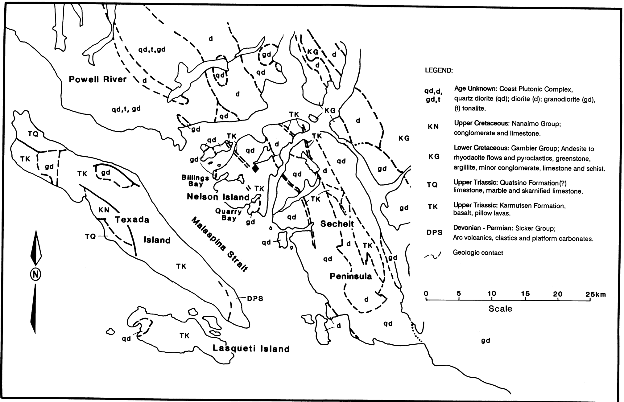
Figure B-x-x. Regional geology (after Roddick and Woodsworth, 1979; Roddick, Muller and Okulitch, 1979) of Nelson Island and area. The location of the skarn occurrence is shown by the diamond.
