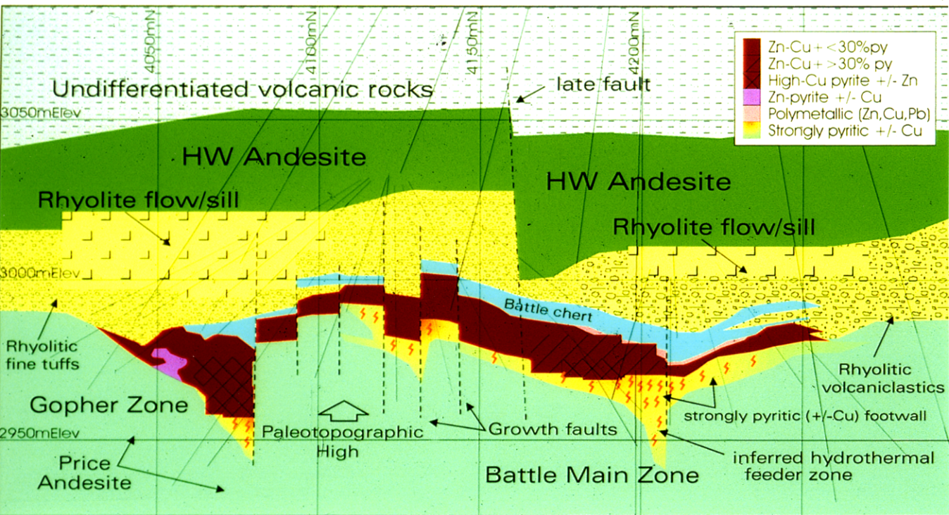
Battle Zone - Geology Section - 1585mE
