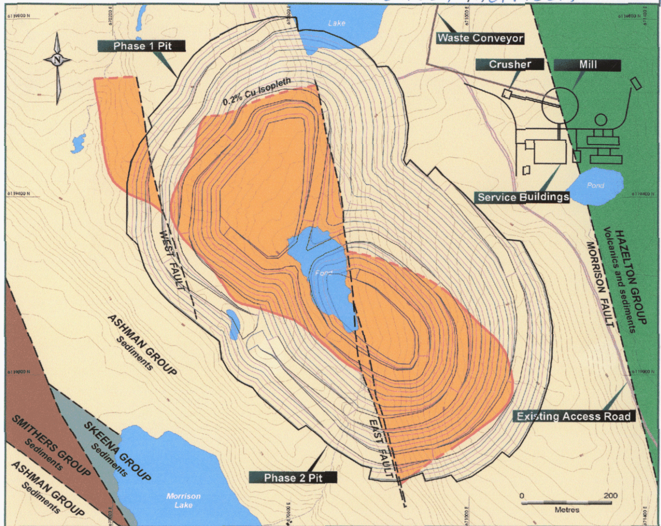
Proposed Mine Layout
