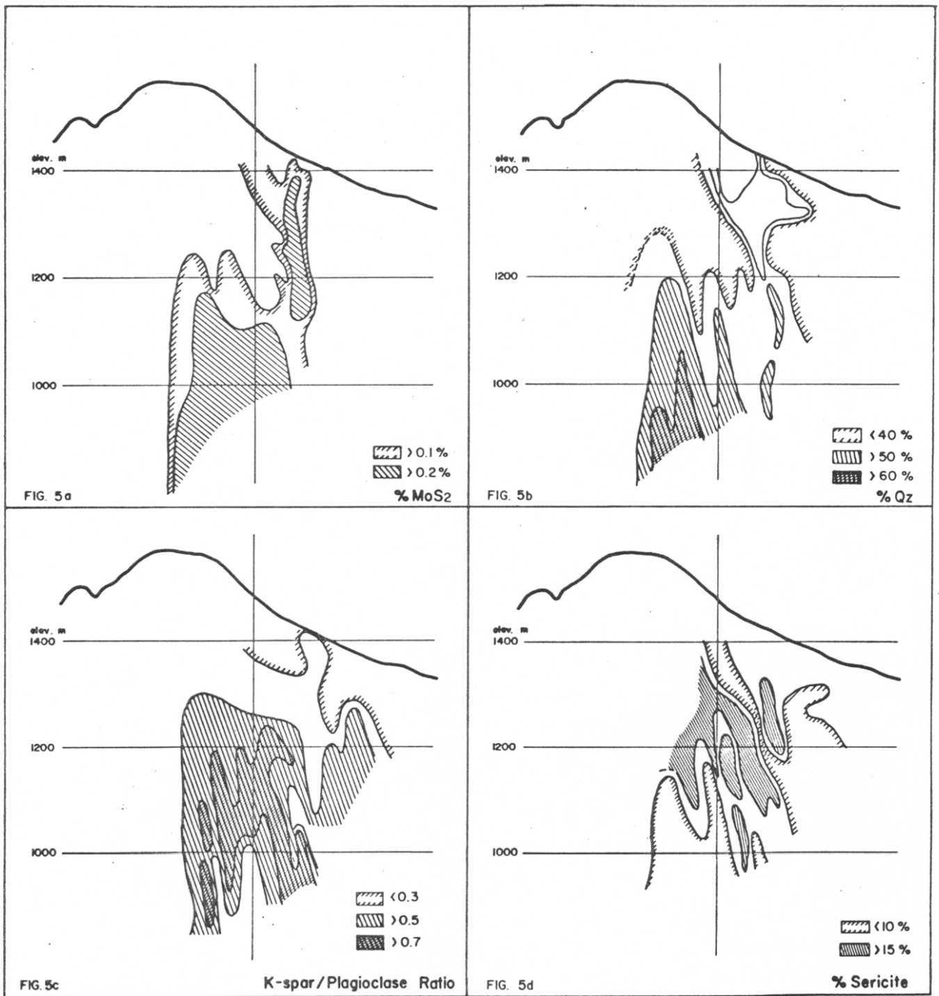
Figure 5 Generalized XRD alteration patterns along section AB
