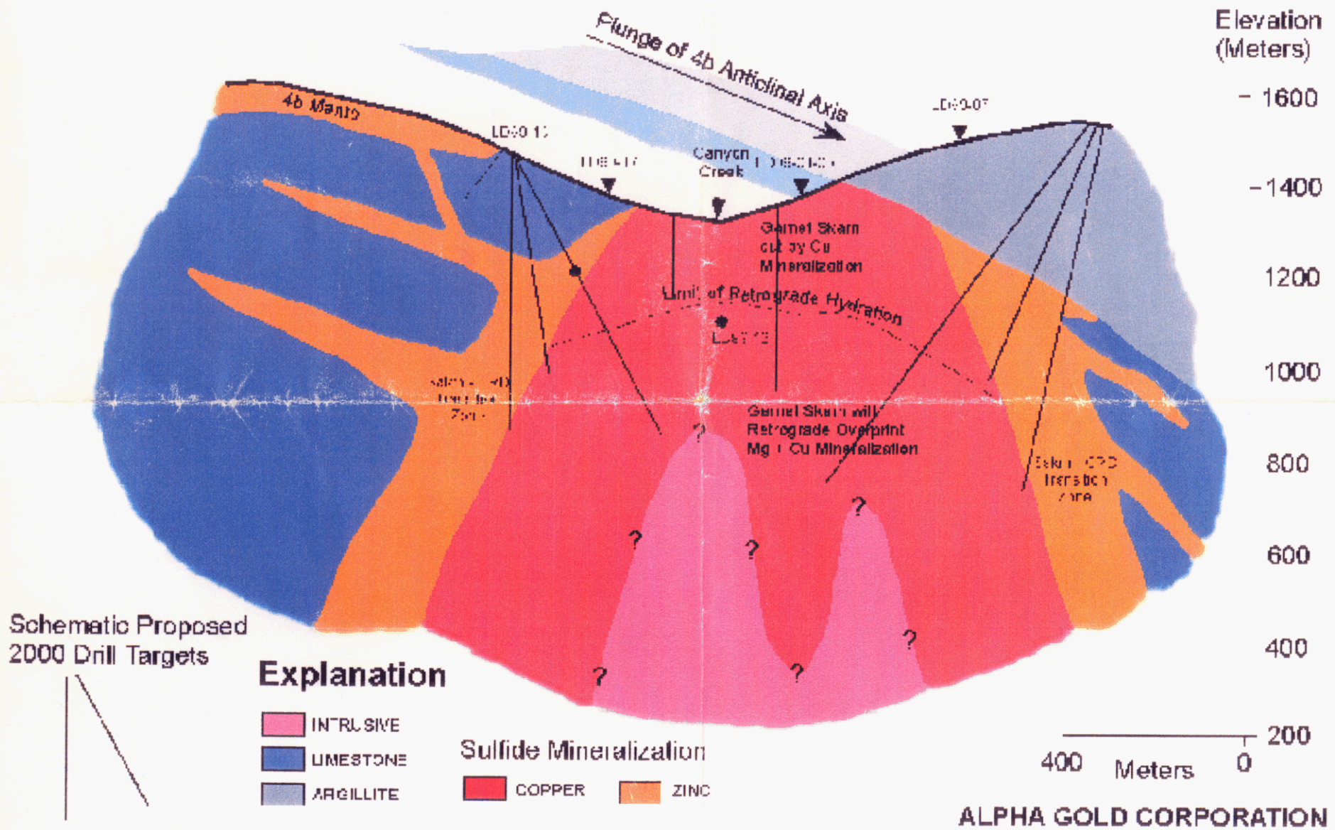
FIGURE 7: Interpretive cross-section through 4b-Canyon Creek Skarn Zone at Lustdust, showing potential drill targets in the Transition Zone adjoining skarn, and in the skarn itself.
