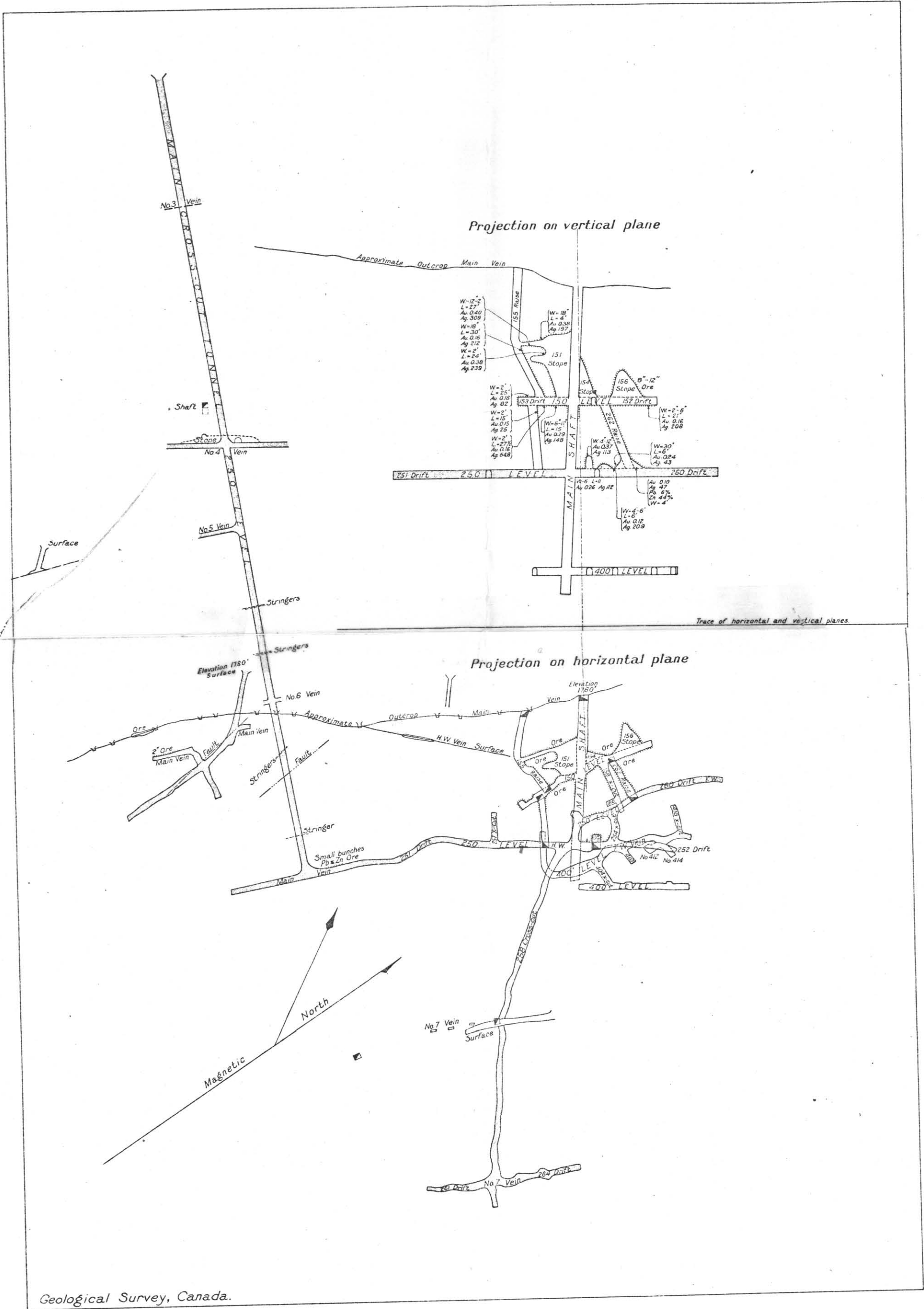
Figure 5. Plan and elevation of main workings, Silver Standard mine, 1917, Hazelton, British Columbia. (By courtesy of Management)
