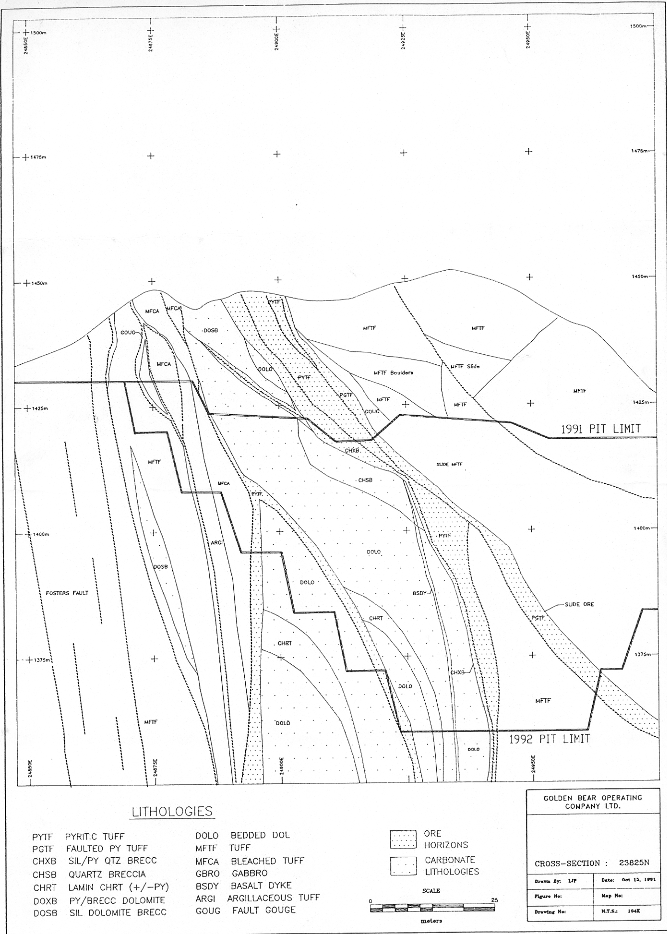
Figure 3.1.1 Idealized cross-section through 23825 N with slide ore projected from 23775 N.
