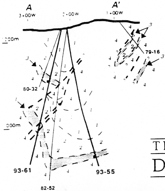
Section 16+00 N (LOOKING GRID NORTH)
