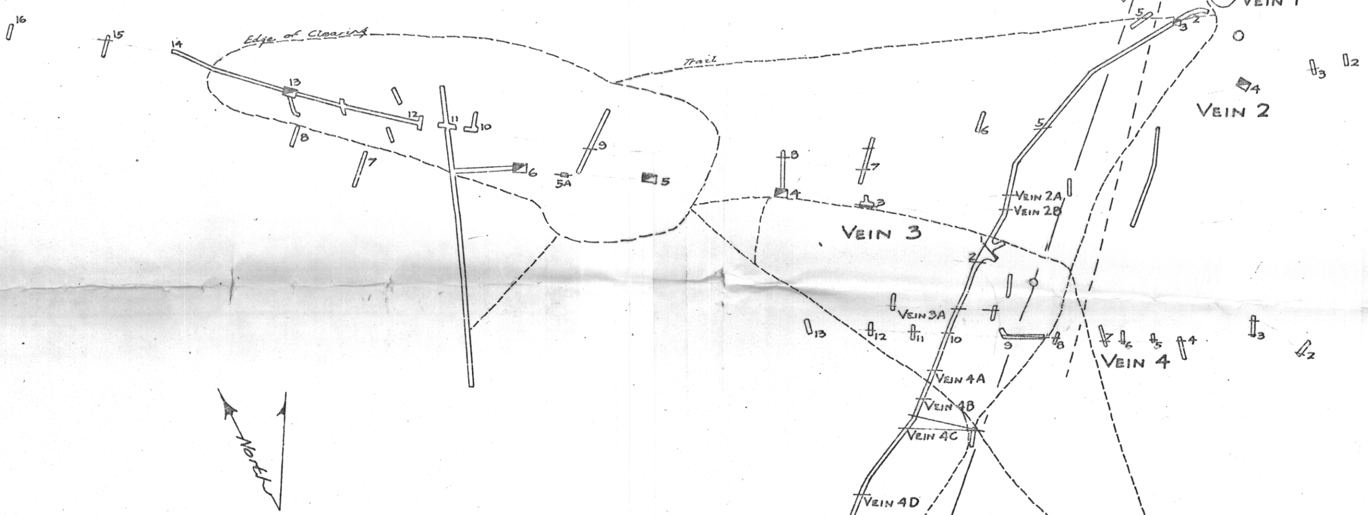
Plan of Surface Work. on FREE GOLD GROUP Dome Mountain, near Telkwa, B.C. Season 1932. Scale: 1"=50'
