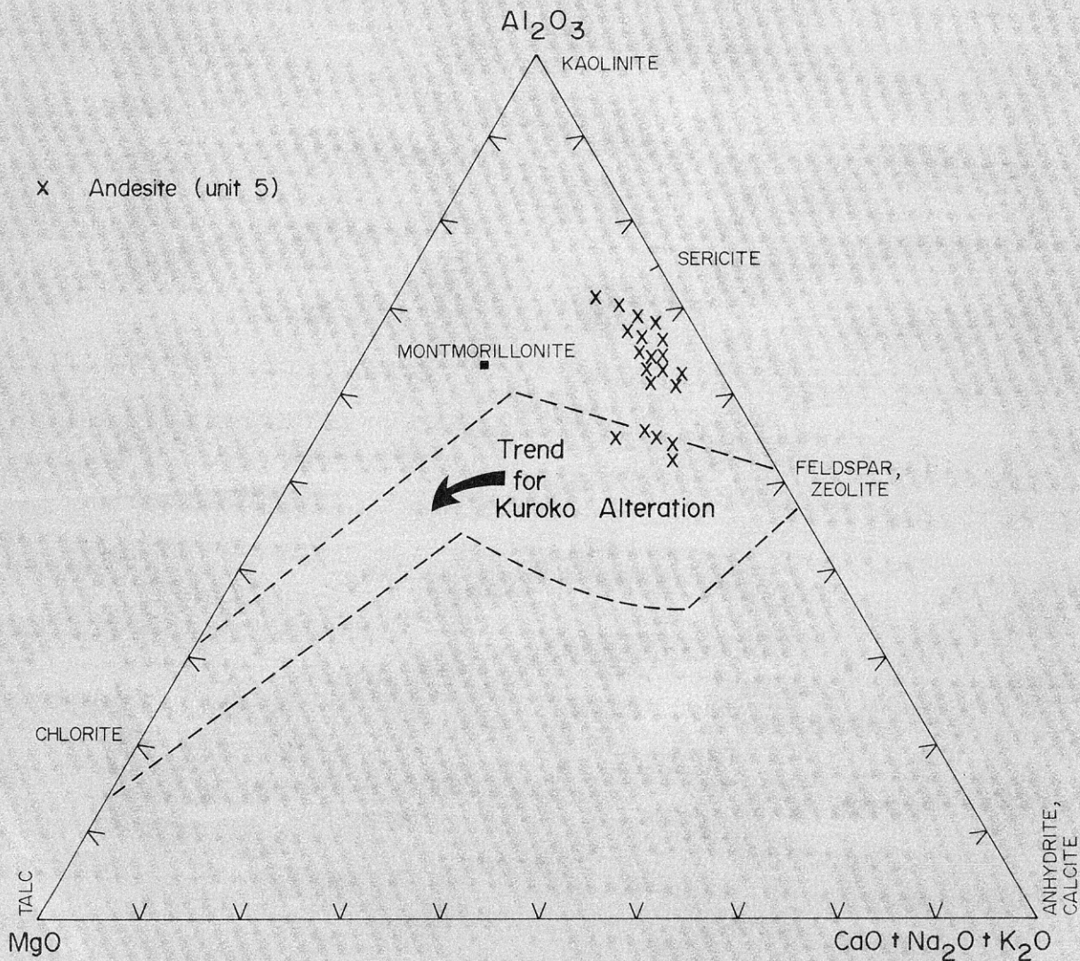
FIGURE 11. Al 2 O 3 - MgO - (CaO + Na 2 O + K 2 O) MOLE PROPORTIONAL DIAGRAM FOR THE BIG MISSOURI ANDESITES
