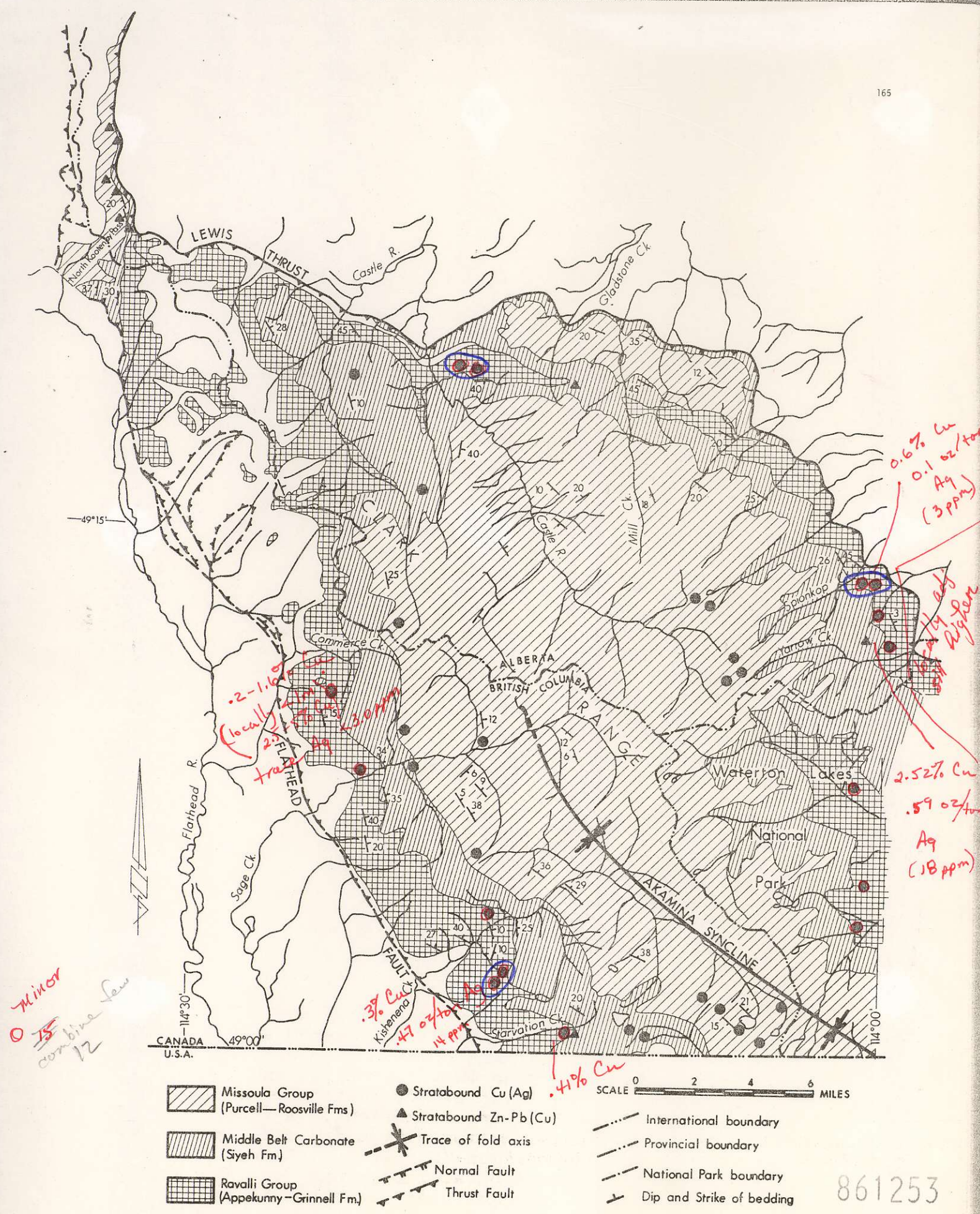
Fig. 3. Geological Sketch Map of Clark Range and locations of principal stratabound Cu (Ag) and Zn-Pb (Cu)
