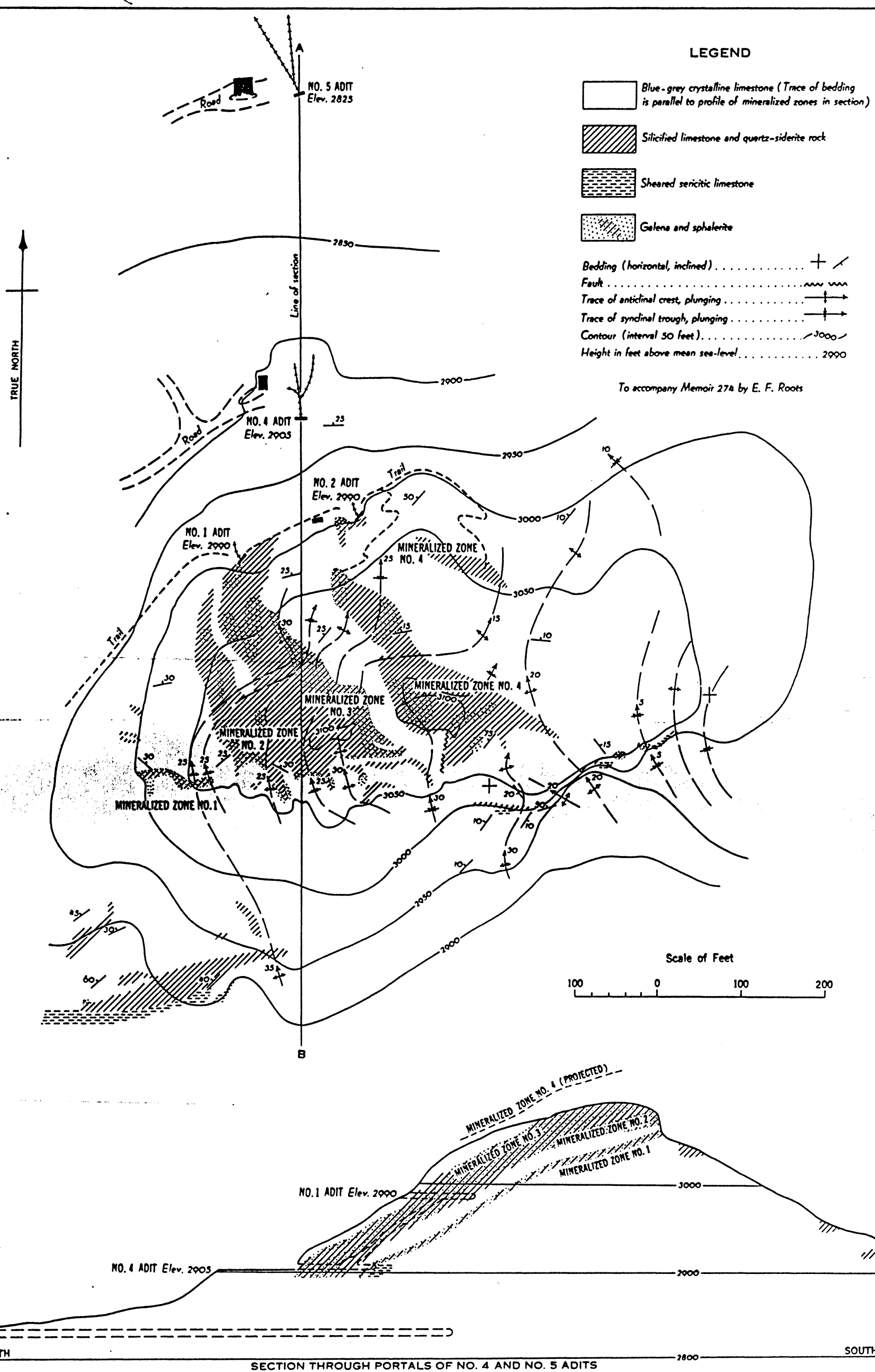
Figure 13 Geological plan and section of the Ferguson property, Ingenika Mines Limited, Aiken Lake map area, British Columbia
