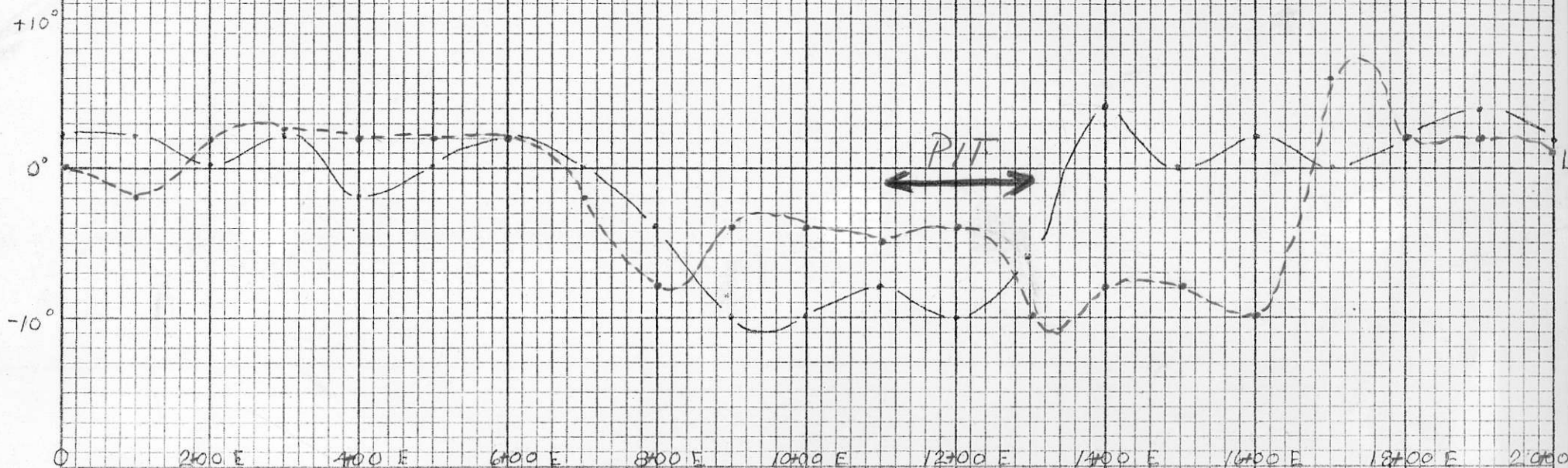
Figure 5 Seneca Property CEM Profile of Resultant Dip Angle Scale 1" = 200' Profile Scale 1" = 10° KWD AVIES
