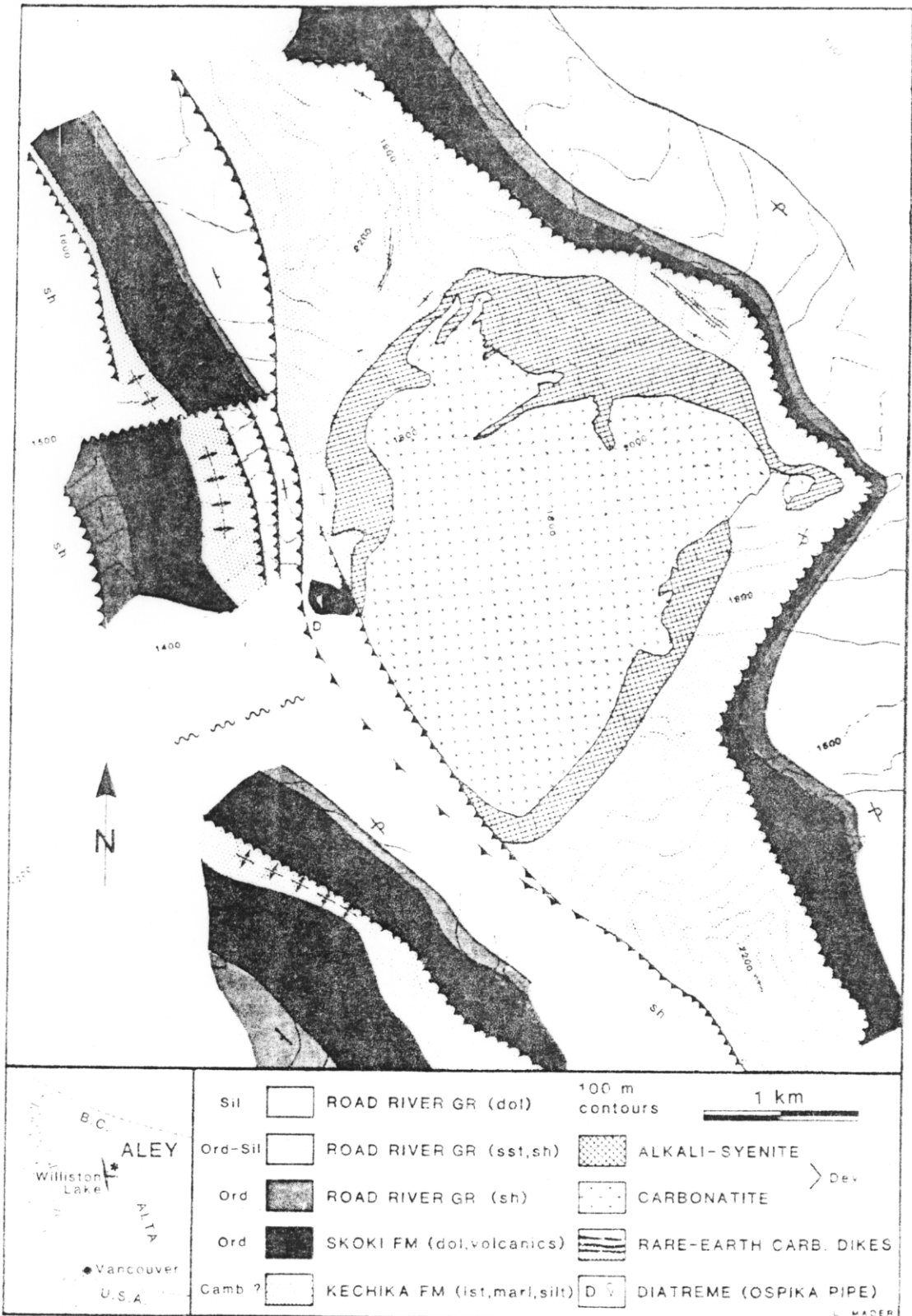
Figure 2. Geological map of the Aley carbonatite complex (from Mäder, 1997).
