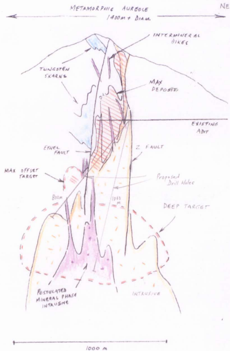
MAX No EXPLORATION MODEL SCHEMATIC SECTION B
