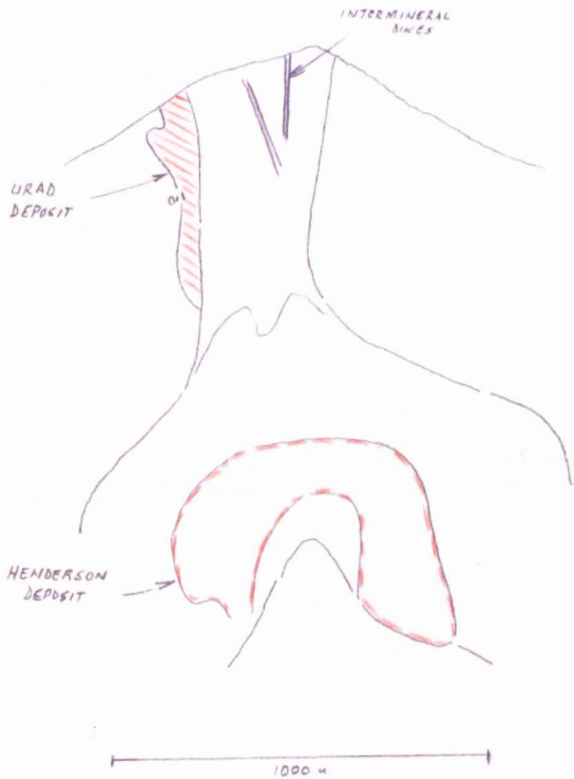
HENDERSON/URAD DEPOSITS SCHEMATIC GEOLOGY (FOR SCALE COMPARISON)
