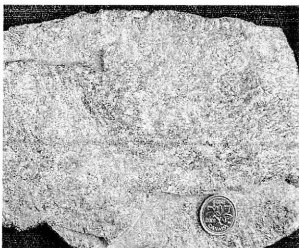
Figure 15: Sulphide mineral textures - Battle and Gap Deposits
