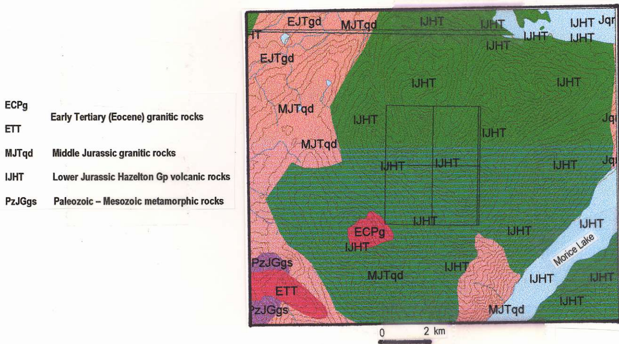
FIGURE 6 - BAY PROPERTY GEOLOGY
