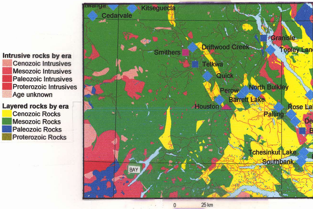
FIGURE 5 - REGIONAL GEOLOGICAL SETTING
