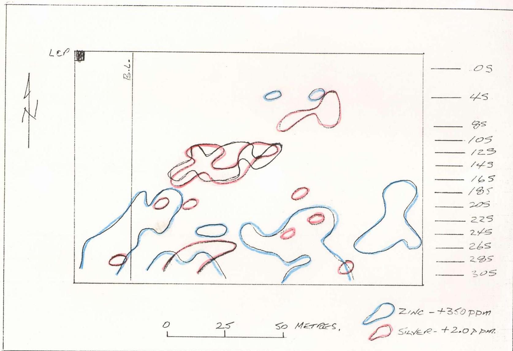
FIGURE 4 - SOIL GEOCHEMISTRY - FORD MINERAL CLAIM.
