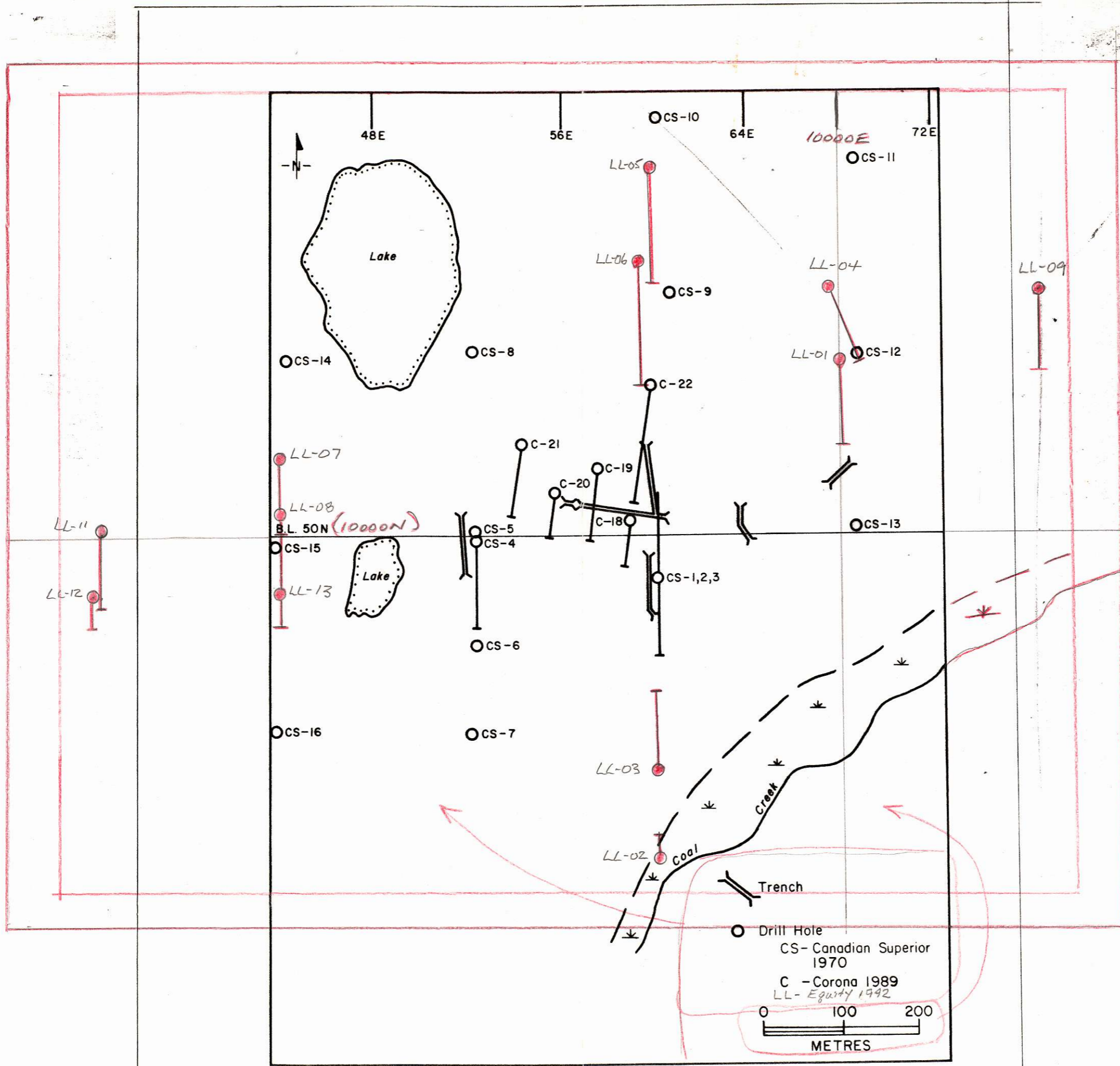
Fig. 5 A Drill Hole Plan
