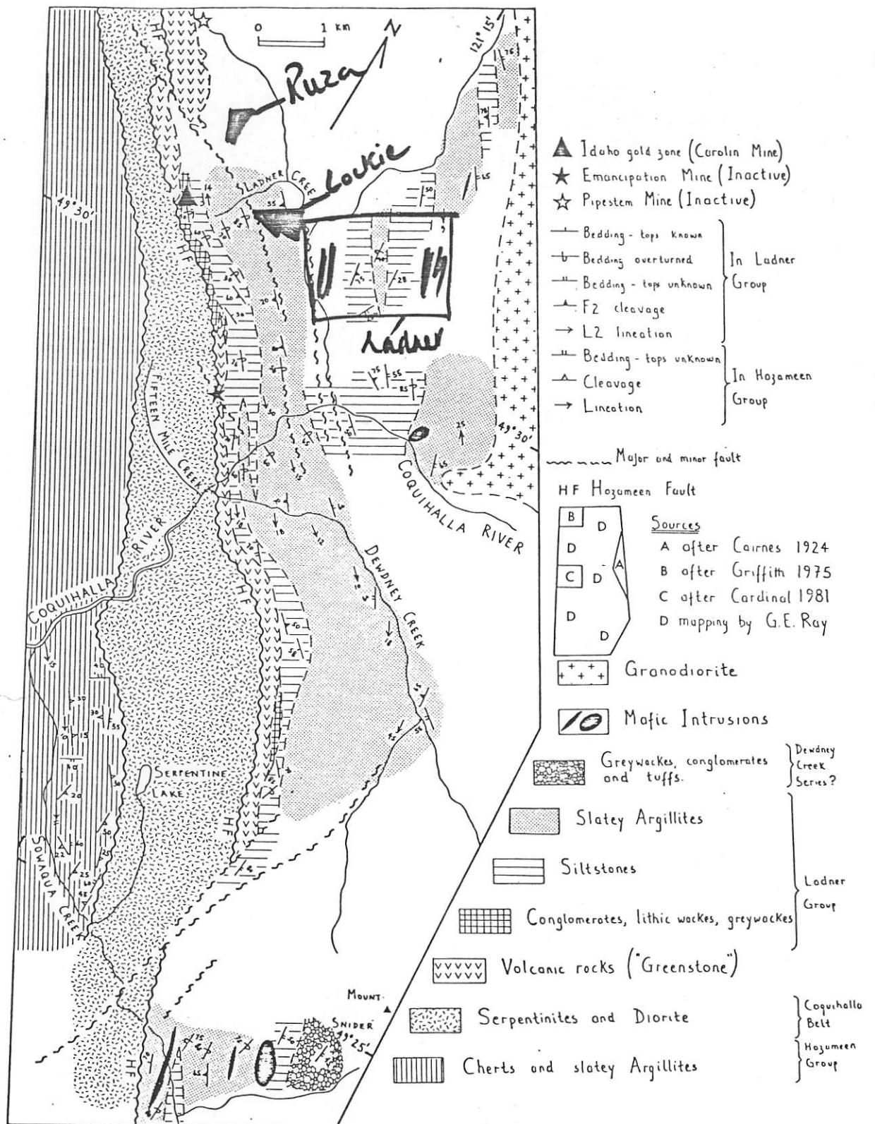
Figure 1. Regional geology of the Coquihalla River area.
