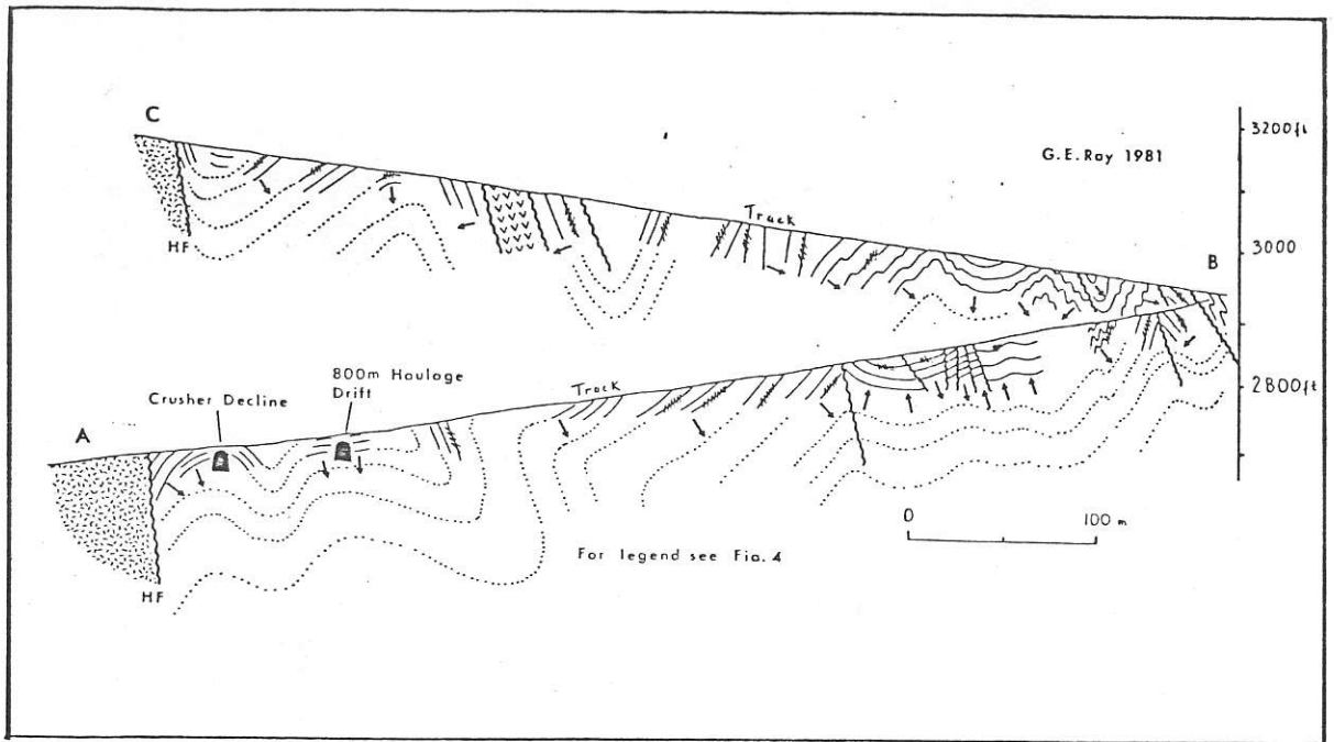
Figure 3. Geological sections AB, BC (see Figure 2) In the Carolin mine area.
