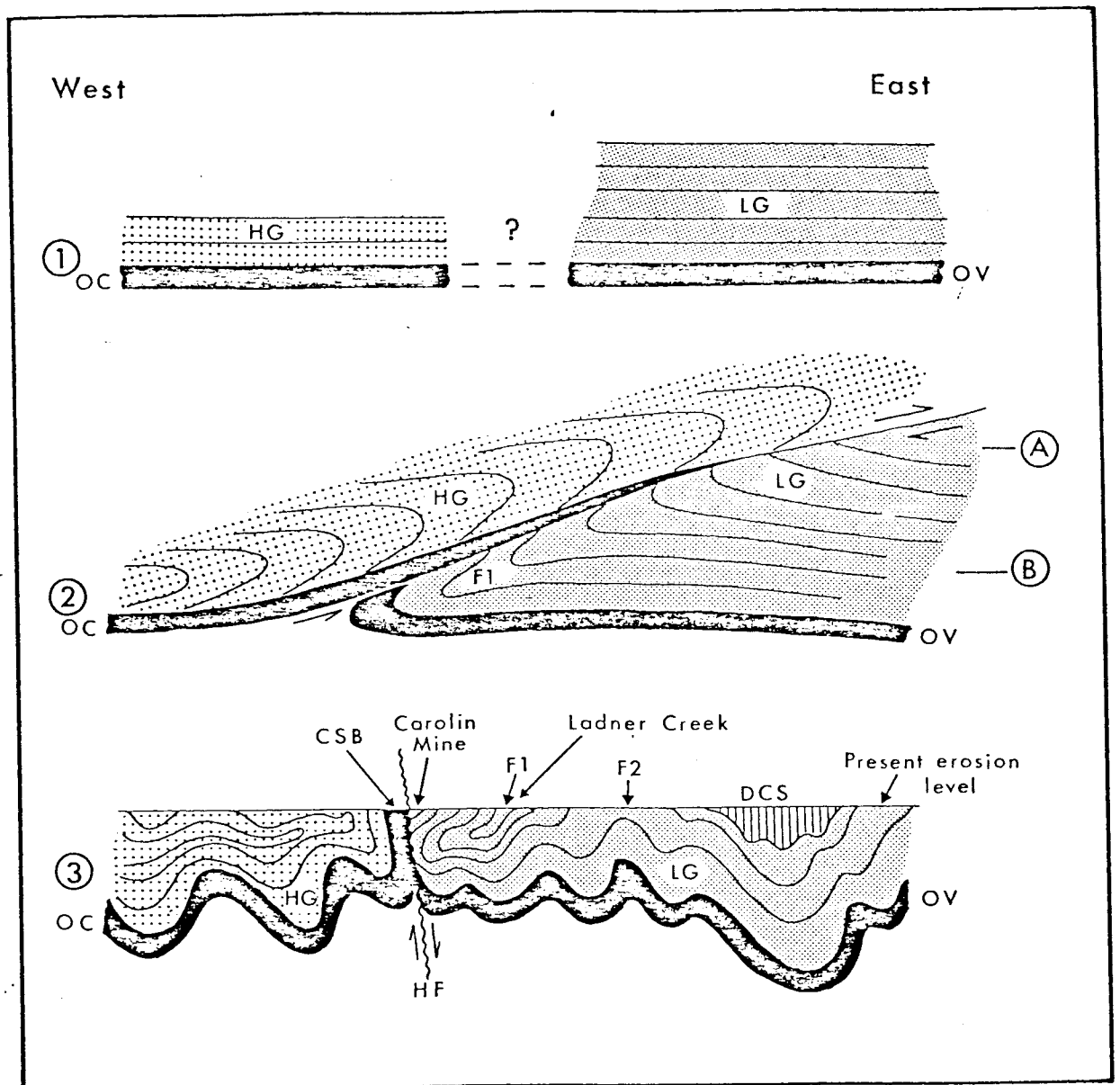
Figure 6. Postulated evolutionary history of the Coquihalla Serpentine Belt:
