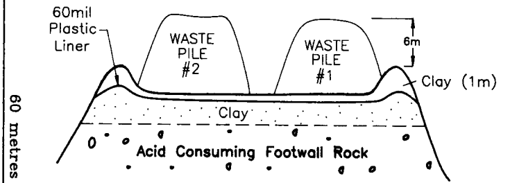
EAST-WEST CROSS SECTION
