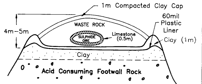
EAST-WEST CROSS SECTION
