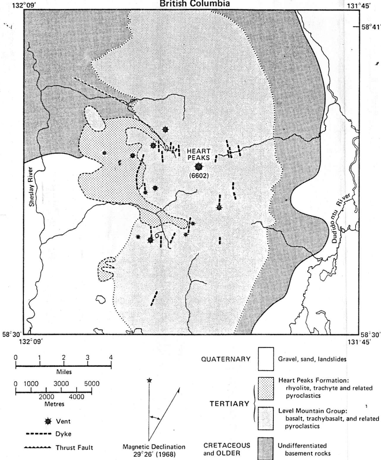
Fig. 4. Geology of the Heart Peaks area.
