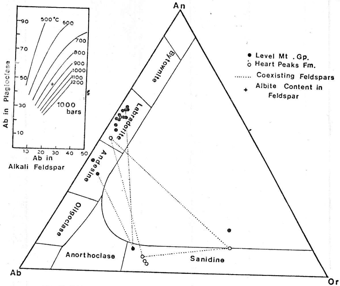
Fig. 16. Feldspar compositions in Heart Peaks volcanics and feldspar geothermometer after Stormer (1975).
