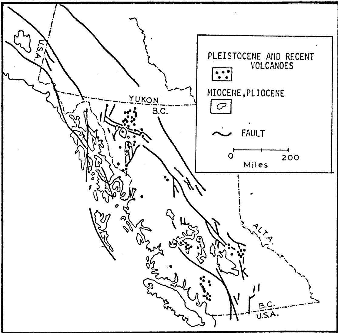
Fig.2. Distribution of late Tertiary and Quaternary volcanic rocks of British Columbia and Yukon Territory.(after Souther,1970)
