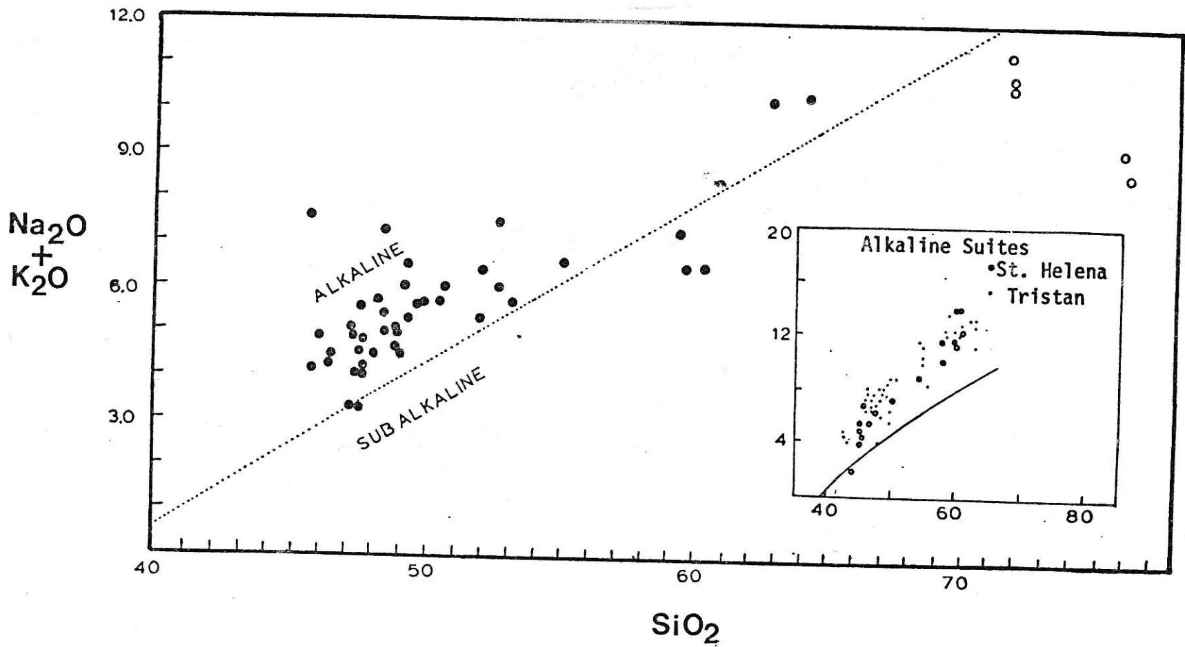
Fig. 7. Silica vs. alkalis diagram, Heart Peaks volcanics. Boundary after MacDonald and Katsura (1964). ○ Heart Peaks Formation. ● Level Mountain Group.
