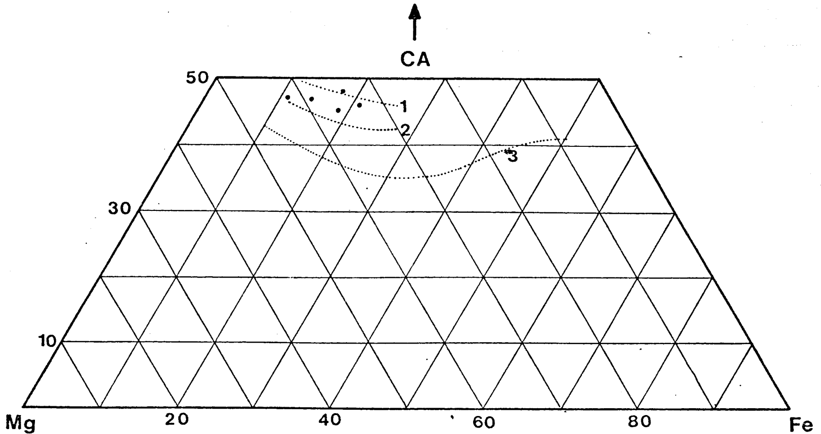
Fig. 17. Pyroxene compositions in Heart Peaks volcanics. Trend 1 - Black Jack Sill, Trend 2 - Garbh Eilean Sill, Trend 3 - Skaergaard. • Level Mountain Group.
