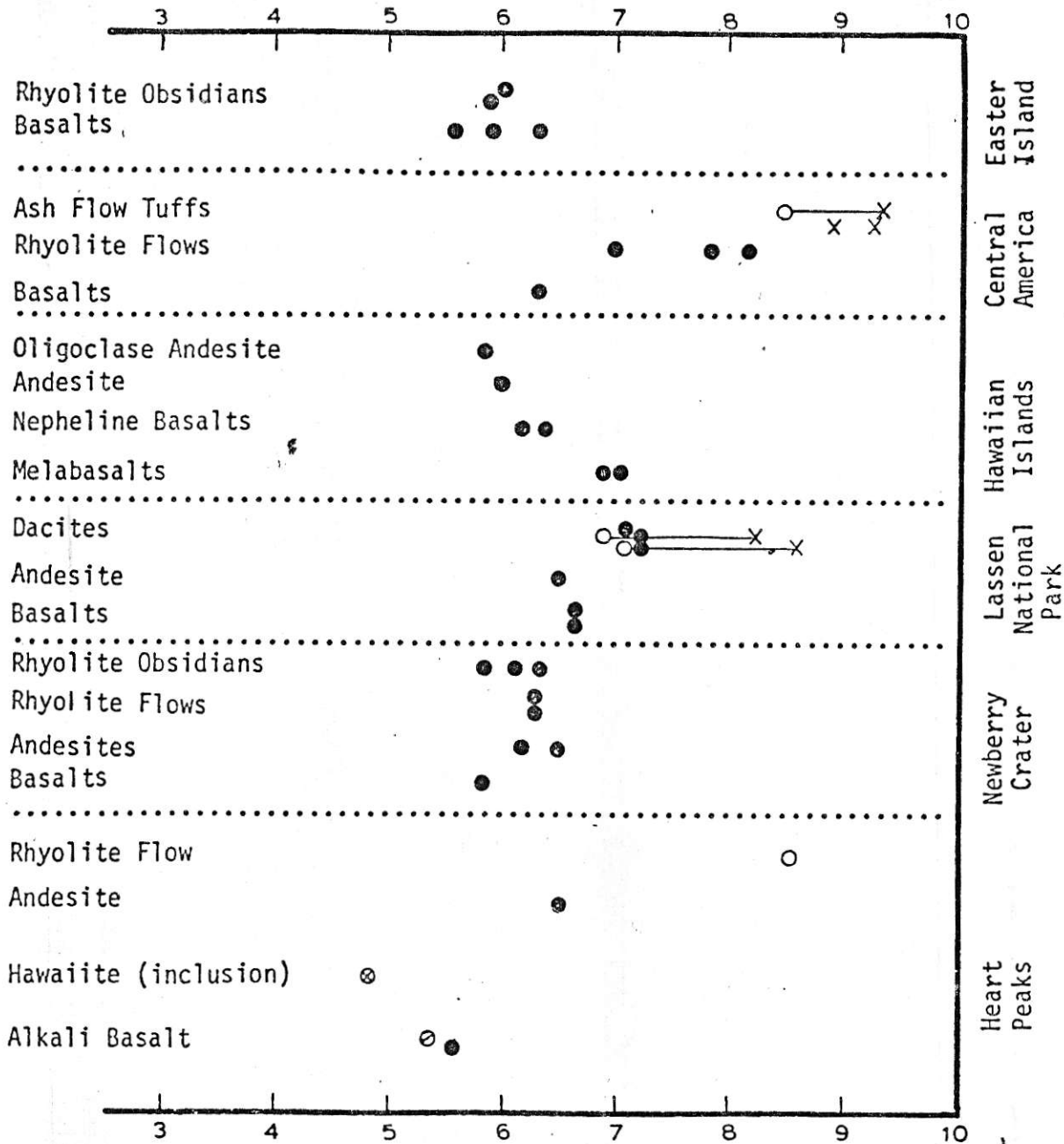
Fig. 15. Graph showing variation of ^{18}\text{O}/^{16}\text{O} in several volcanic centres compared to Heart Peaks centre. O Feldspar. X quartz. ⊙ hornblende. ⊘ pyroxene. ● whole-rock. Other data from Taylor(1968).
