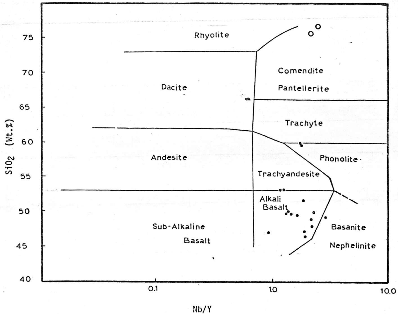
Fig. 13. Classification of volcanics using immobile elements. ○ Heart Peaks Formation ● Level Mountain Group Boundaries after Winchester and Floyd (1977).
