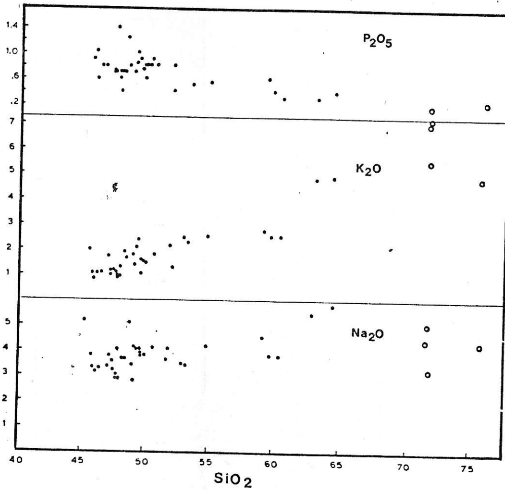
Fig. 11. Major element variation diagrams, Heart Peaks volcanics. • Level Mountain Group ● Heart Peaks Formation
