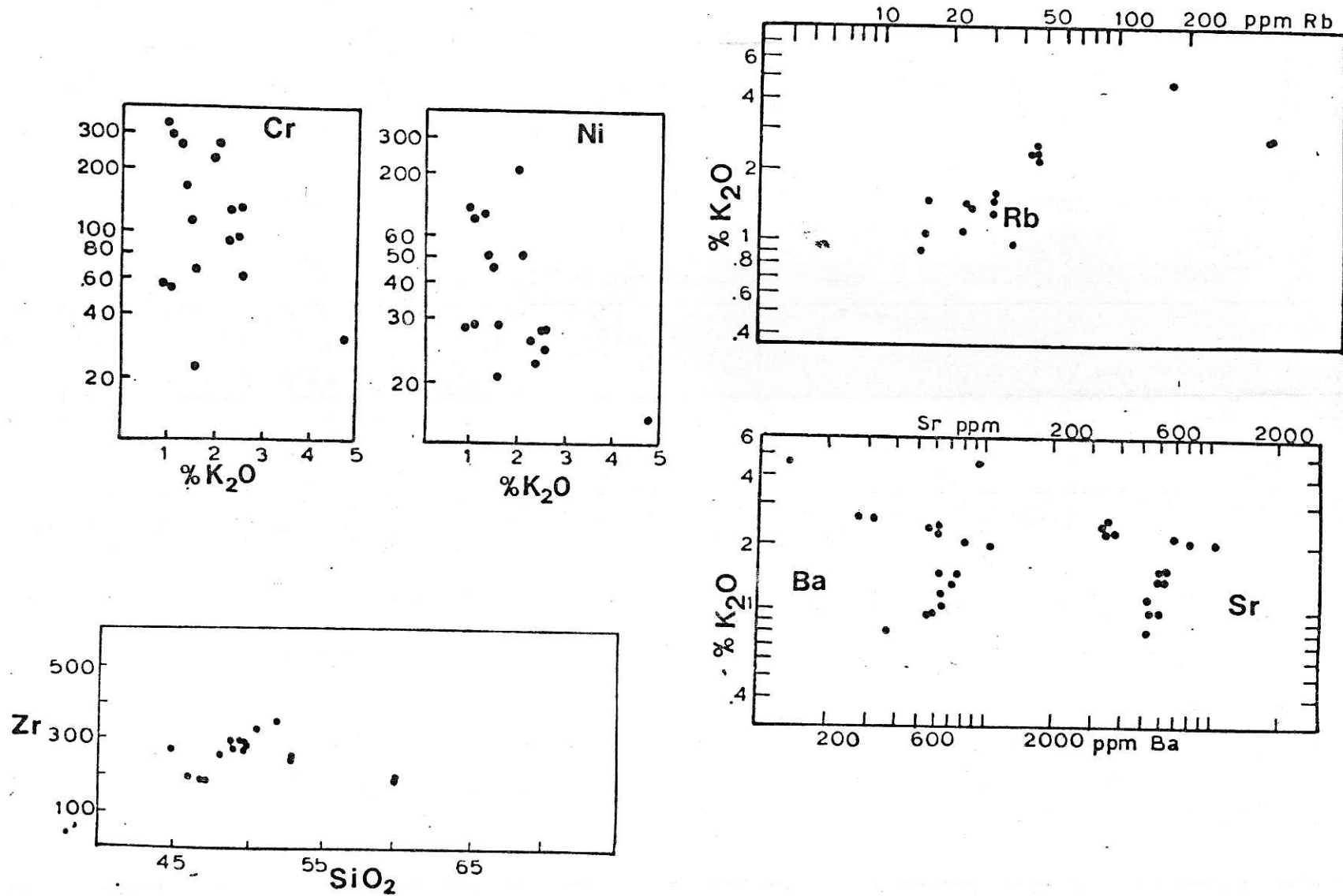
Fig. 14 . Trace element variation in Level Mountain Group rocks.
