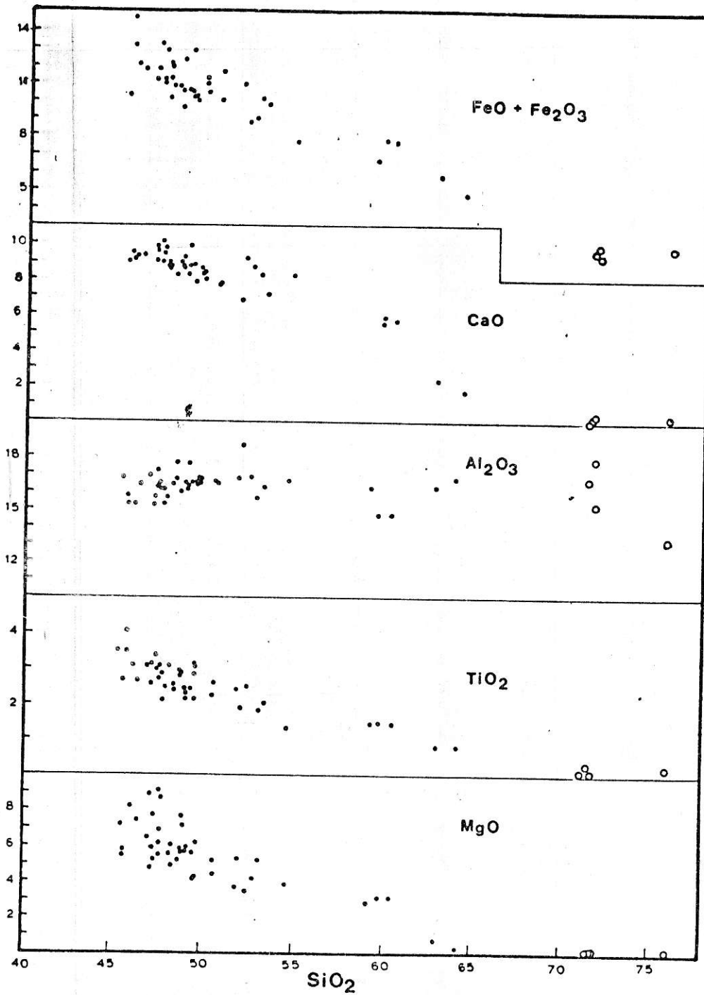
Fig. 10. Major element variation diagrams, Heart Peaks volcanics. • Level Mountain Group ○ Heart Peaks Formation
