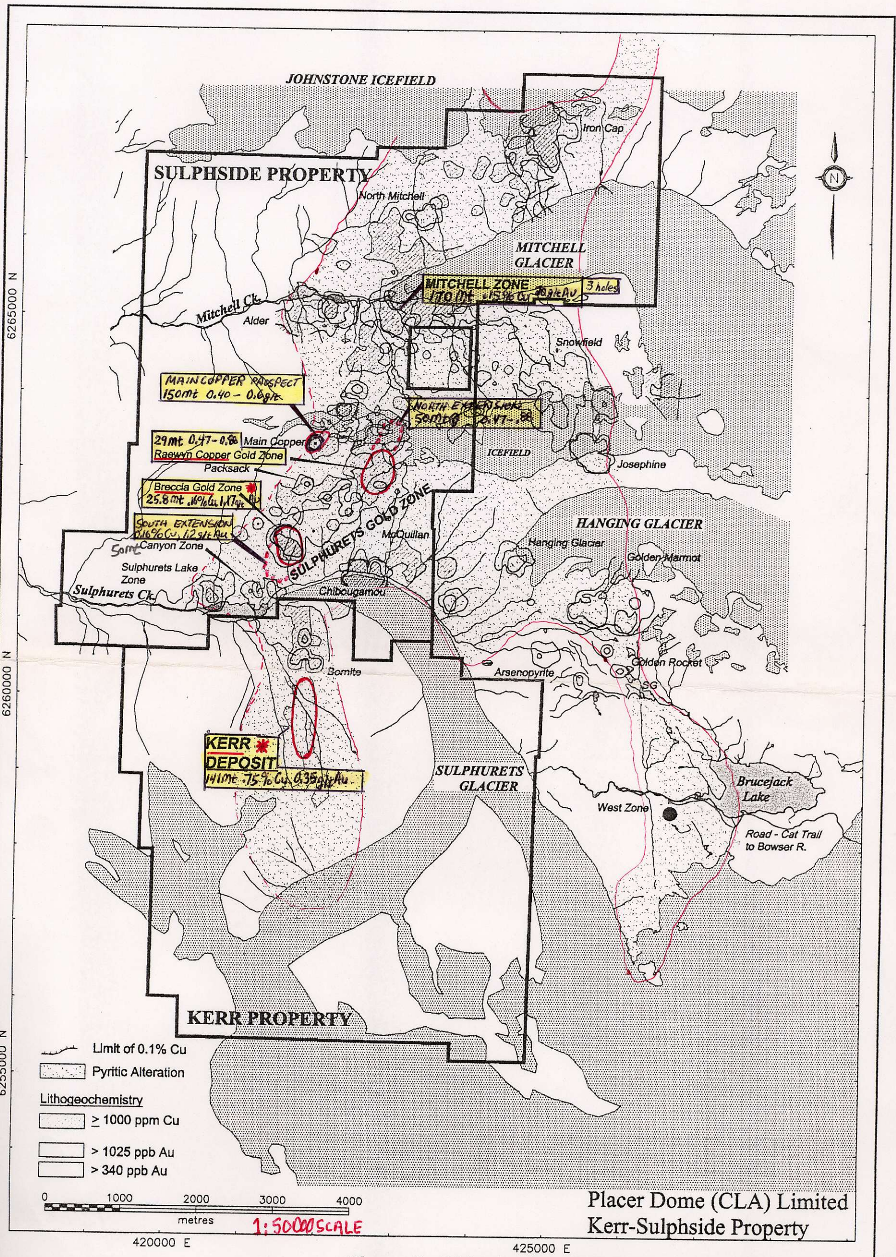
Figure 5: Lithogeochemical & Target Compilation Map
