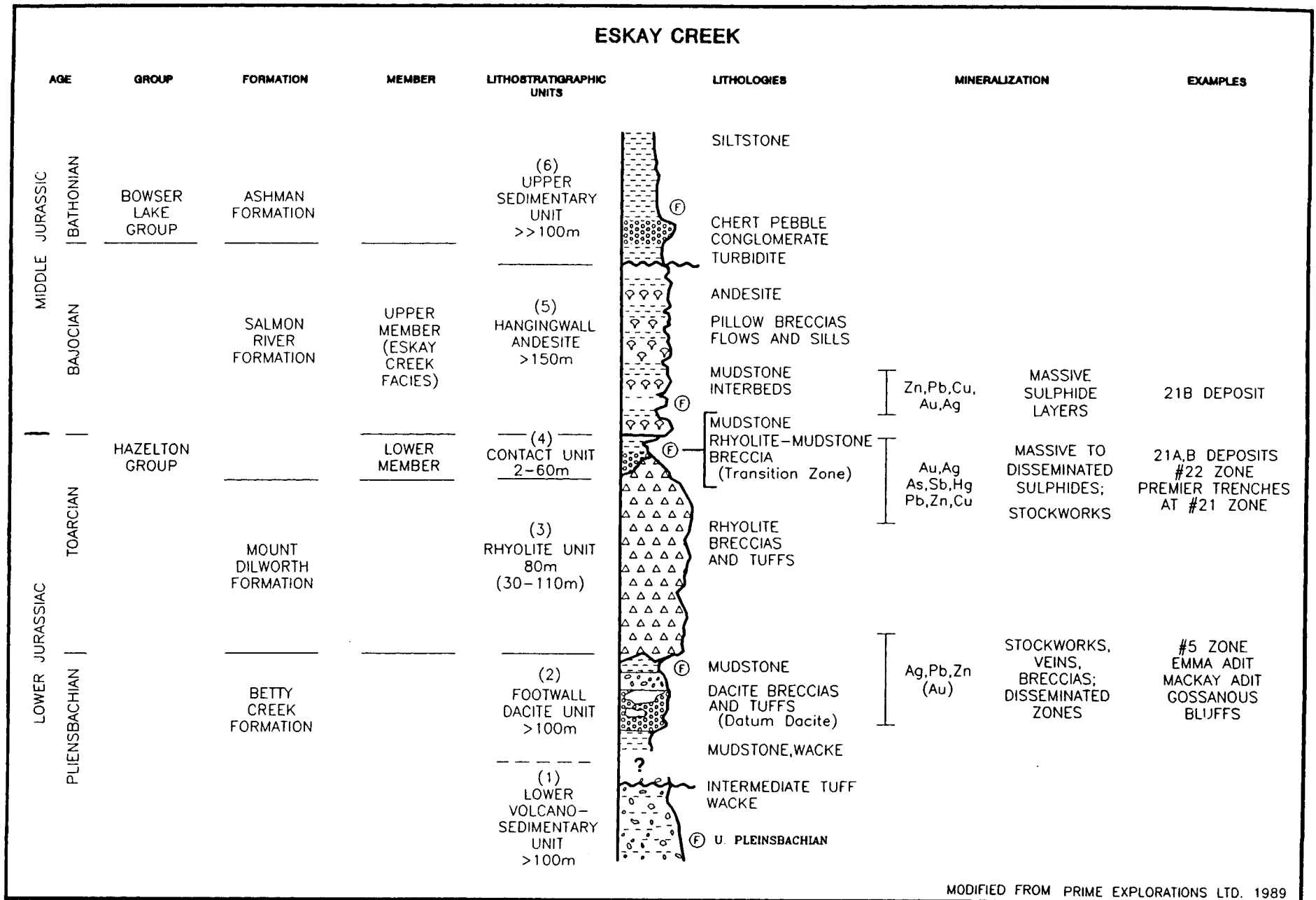
Figure B-14-4. Stratigraphy and mineralization, Eskay Creek.
