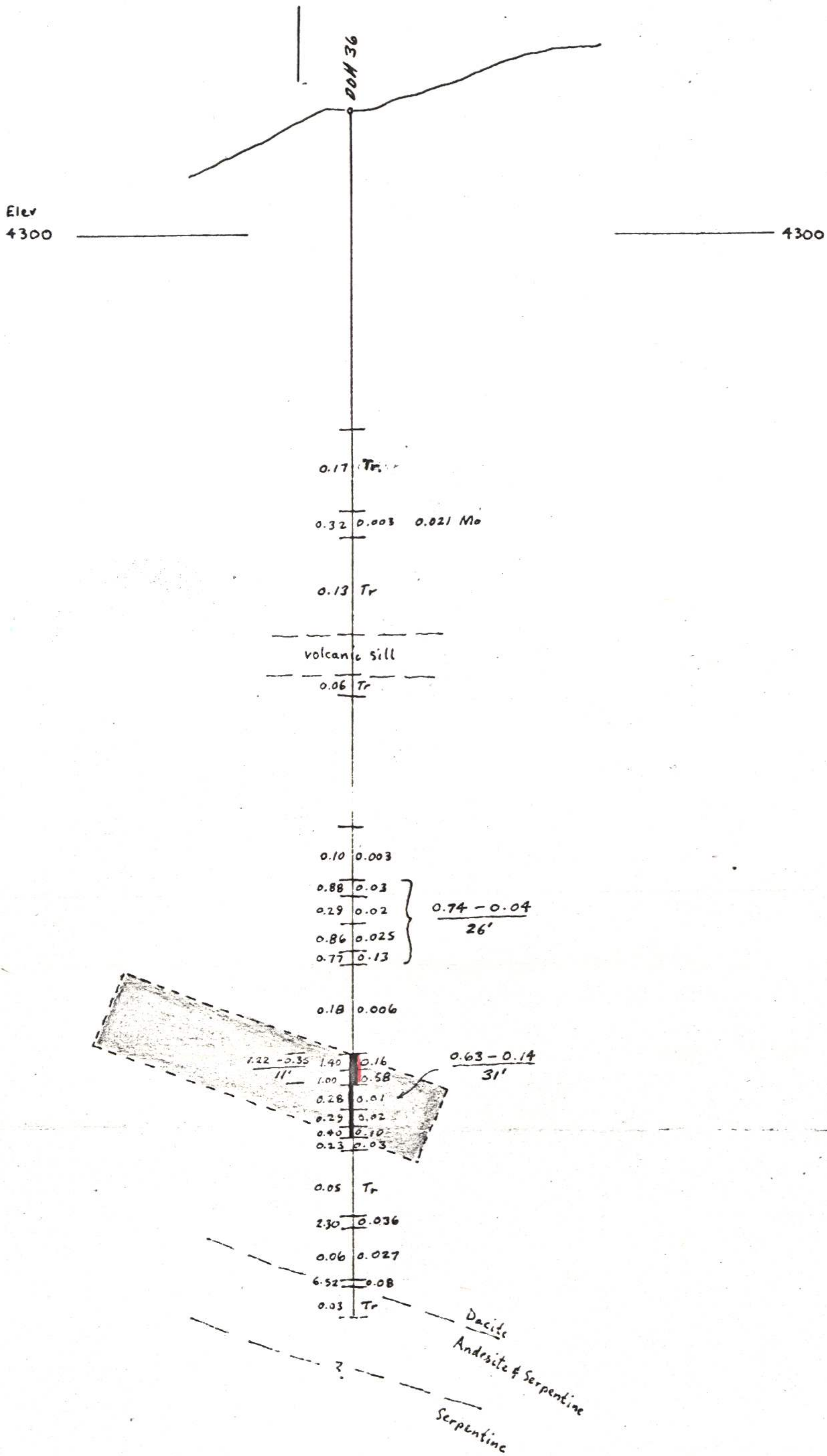
SECTION 16+43N LOOKING NORTHWEST 1" = 50'
