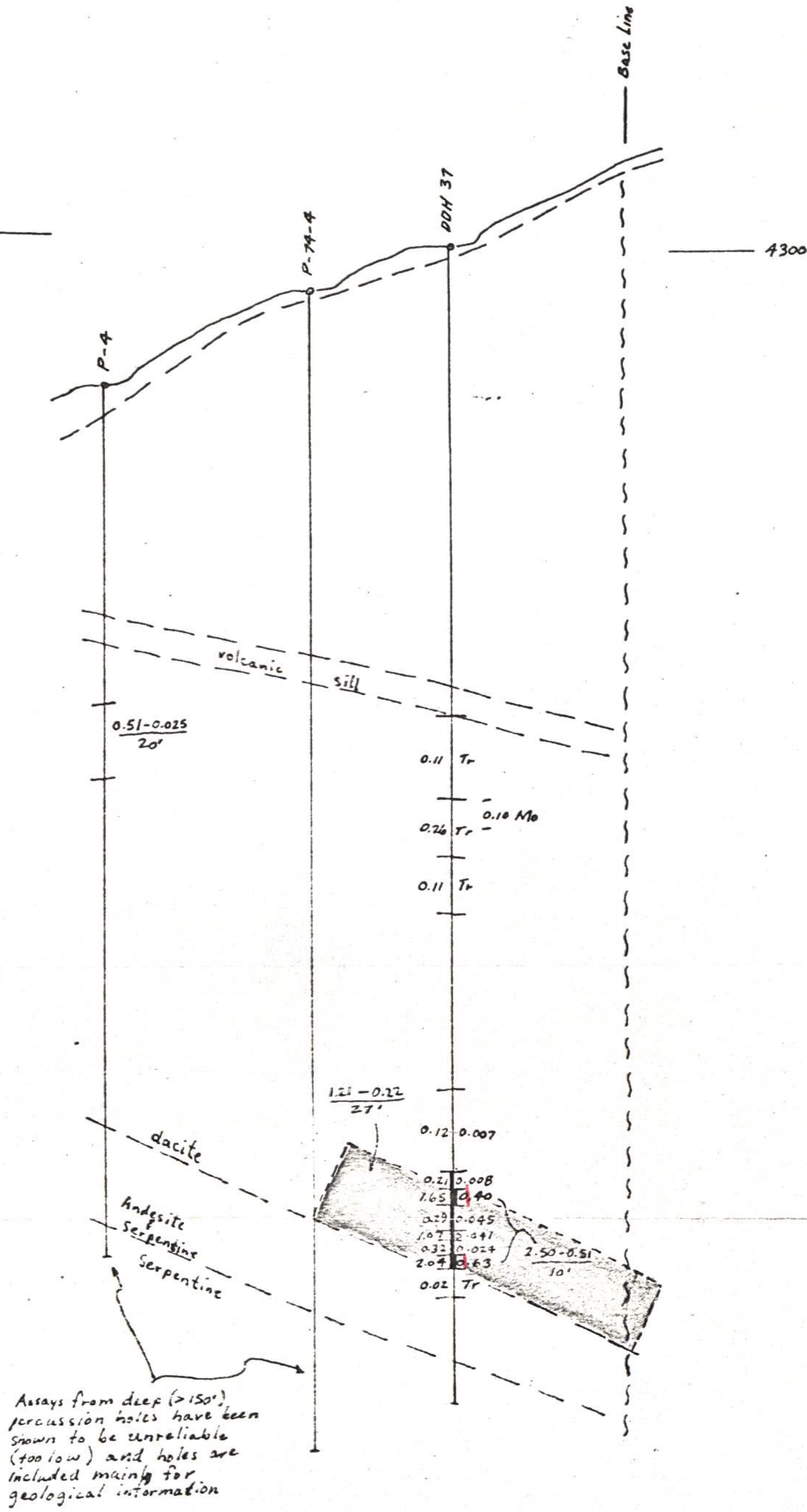
SECTION 13+13N LOOKING NORTHWEST 1" = 50'
